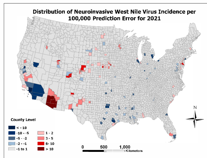
Figure 2: WNV Incidence per 100,000 Prediction Error for the Year 2021
