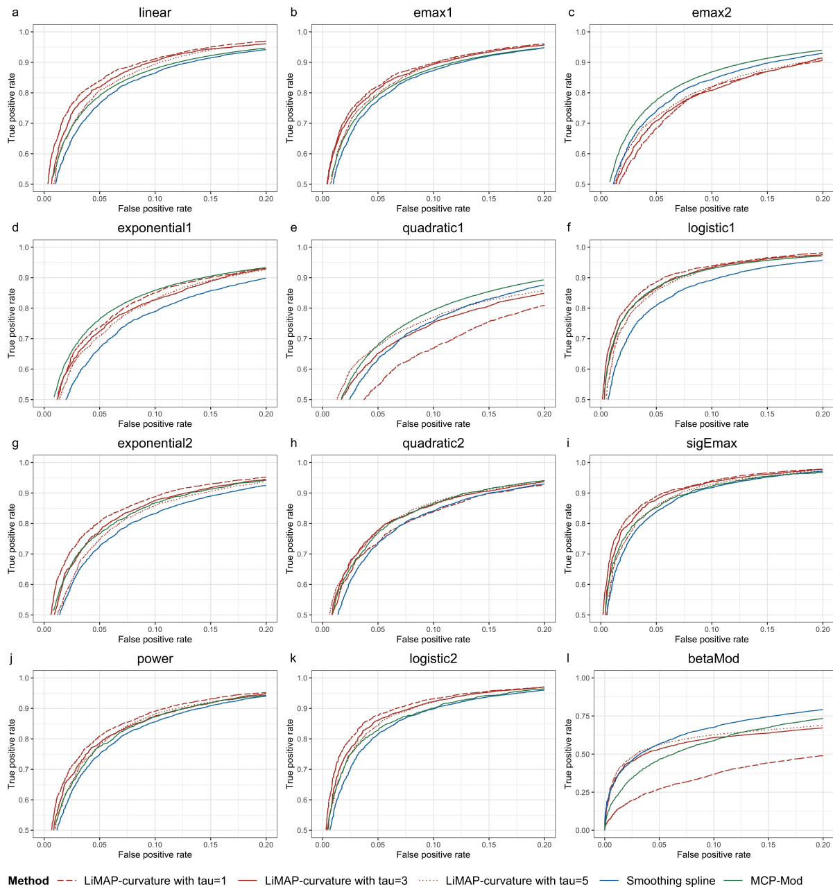
Figure 2: ROC curves of LiMAP-curvature, smoothing spline and MCP-Mod across different true dose-response models with the sample size of 40 patients per arm. The ROC curves of MCP-Mod in (a)-(f) are produced with the true dose-response model not included in the candidate model set, and the ROC curves of MCP-Mod in (g)-(l) are produced with the true dose-response model not included in the candidate model set.
