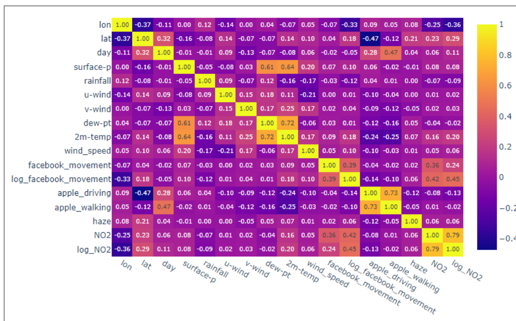
410 Figure 15. Correlation matrix between any pair of variables.
