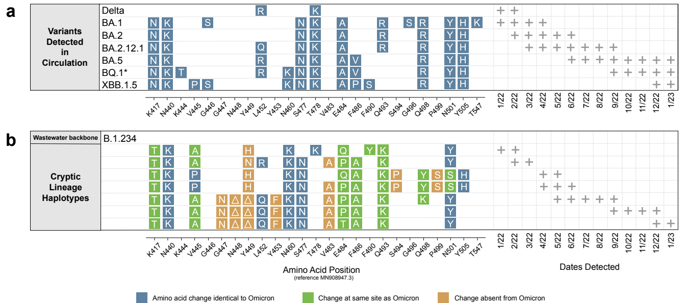
Figure 2. Representative haplotypes of Wisconsin Lineage sequences. (a) The SARS-CoV-2 spike RBD was amplified from Sub-District 5 wastewater samples using primers designed to exclude Omicron lineages. A single amplicon, spanning spike amino acid residues 377-606, was sequenced, and the amino acid changes (relative to Wuhan-1) found in Omicron lineages are shown in blue. (b) Representative haplotypes are displayed, each of which represented at least 25% of the total sequences in at least one sample. Green boxes indicate residues that are also altered in Omicron (BA.1 or BA.2), blue boxes indicate residues that have identical mutations to Omicron lineages, and tan boxes indicate residues that are altered in the Wisconsin Lineage and not in major Omicron lineages. \Delta indicates an in-frame amino acid deletion.
