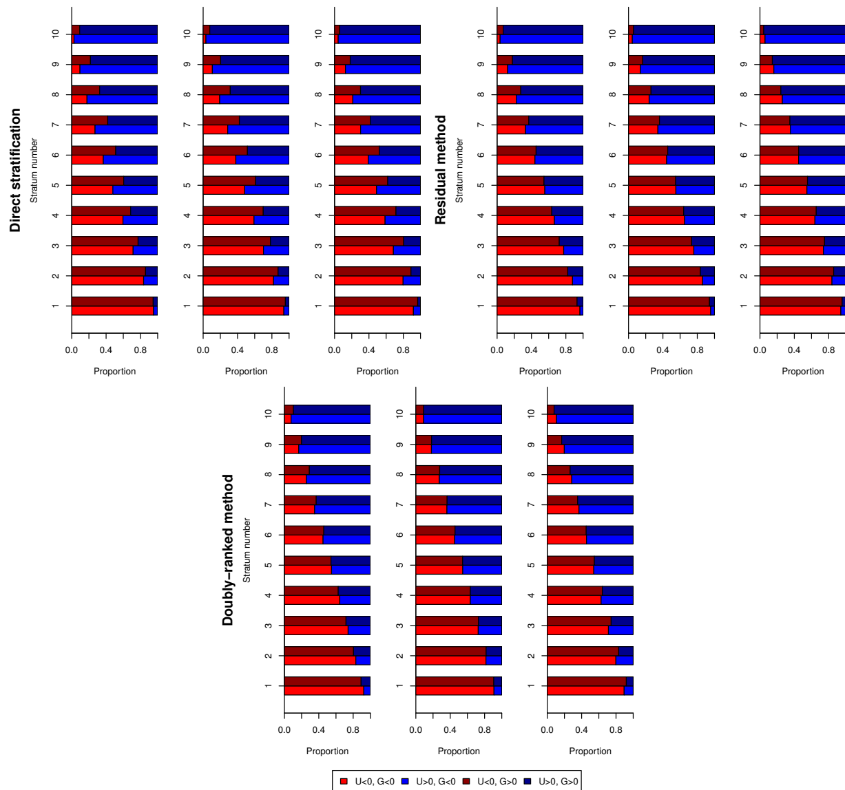
Figure 3: Simulation study 2 results, indicating the proportion of individuals in each genetic group ( G < 0 , brighter colours; or G > 0 , darker colours) for each stratum with the confounder below ( U < 0 , red) or above ( U > 0 , blue) its median value. Strata are defined by stratification on the exposure directly (top-left panel), the residual exposure (top-right panel) or using the doubly-ranked method (bottom panel). For each stratification method, results are presented in three scenarios (left-to-right): 1) genetic effect depends on X only, 2) genetic effect depends on X and U , and 3) genetic effect depends on U only.
