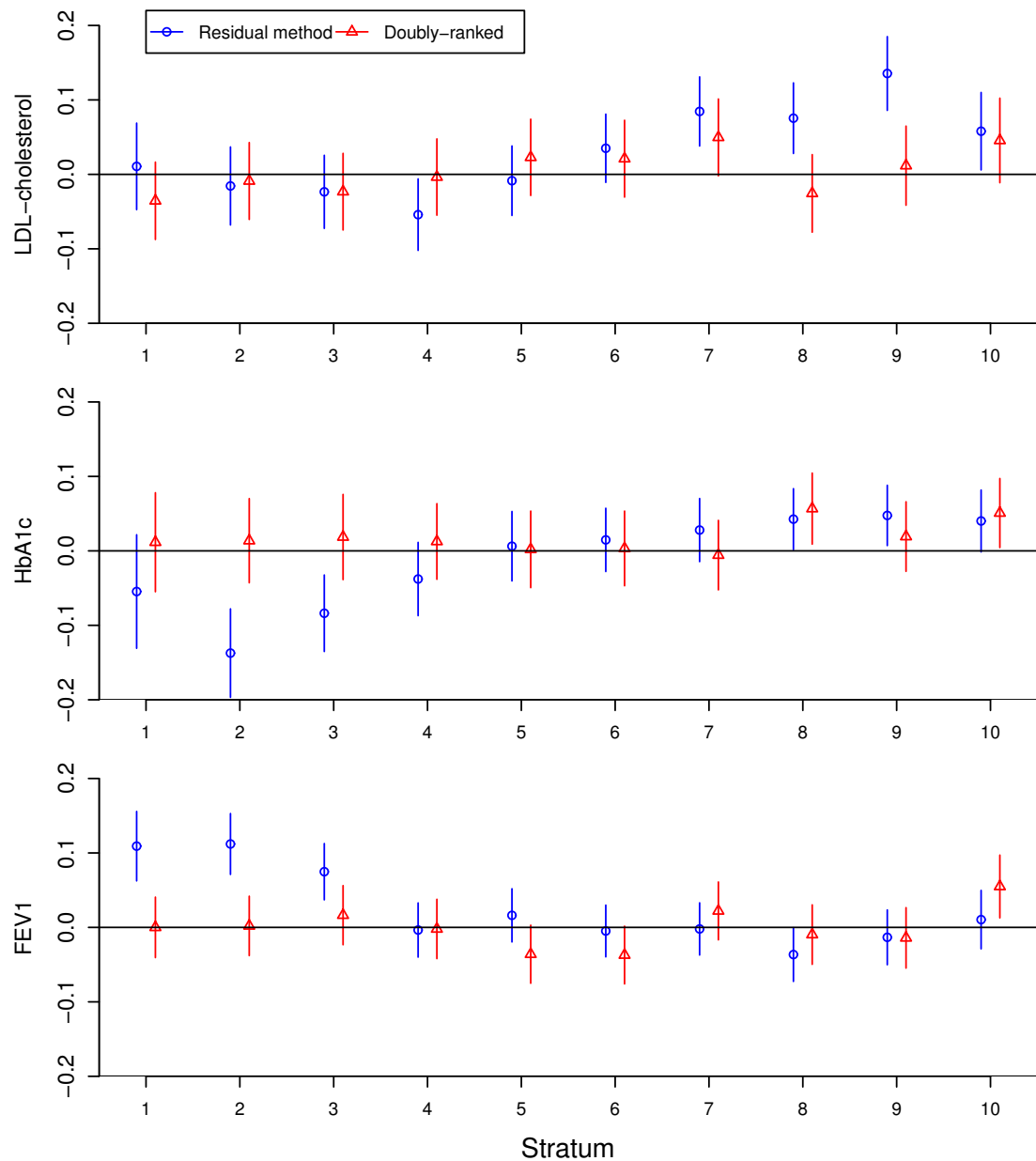
Figure 4: Genetic associations with covariates in strata defined by the residual method (blue circles) and doubly-ranked method (red triangles). Estimates represent associations with the covariate in standard deviation units per unit change in the genetic instrument, corresponding to a standard deviation change in 25(OH)D concentrations. Error bars are 95% confidence intervals.
