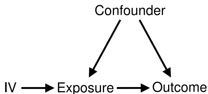
Figure 1: Directed acyclic graph of instrumental variable (IV) assumptions
