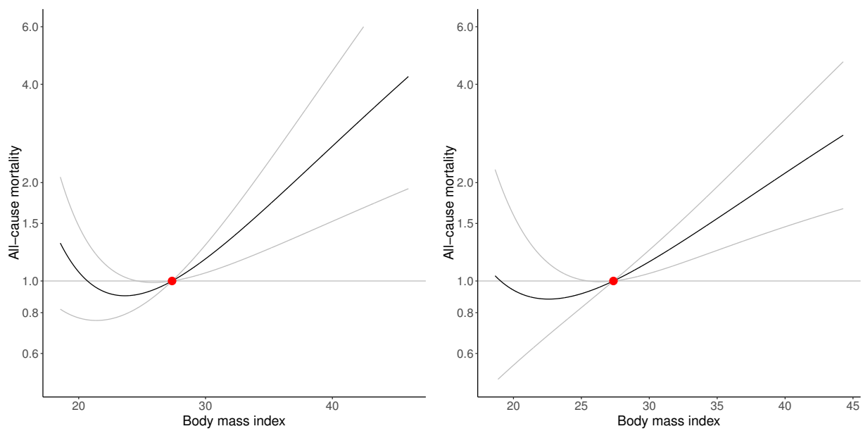
Figure 5: Estimated localized average causal effect curve of body mass index (BMI, \text{kg}/\text{m}^2 ) on odds of all-cause mortality from non-linear Mendelian randomization using fractional polynomial smoothing taking estimates from: (left) the residual method, and (right) the doubly-ranked method. Grey lines represent the 95% confidence interval for the localized average causal effect curve.
