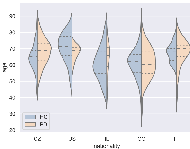
Figure 2: Probability distribution of age.
