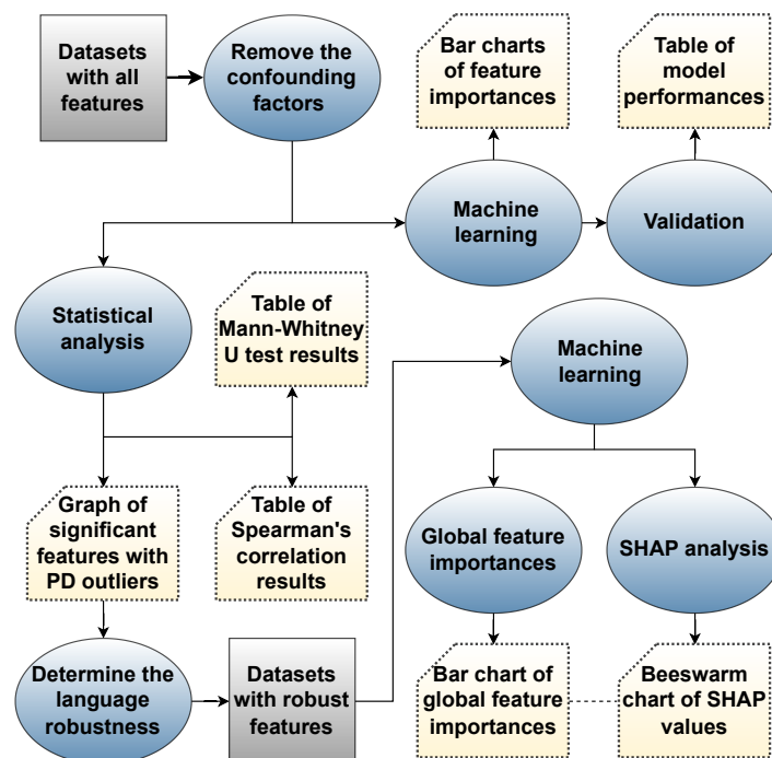
Figure 1: Workflow.
