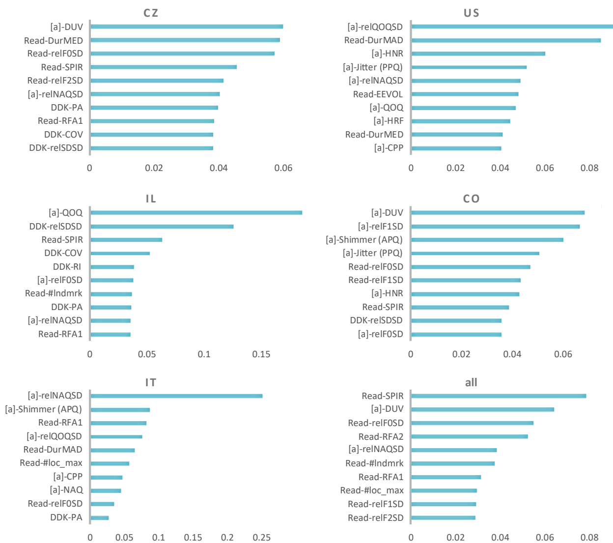
Figure 4: Coefficients of importance of ten most important features in each language scenario (machine learning models trained by all extracted features).
