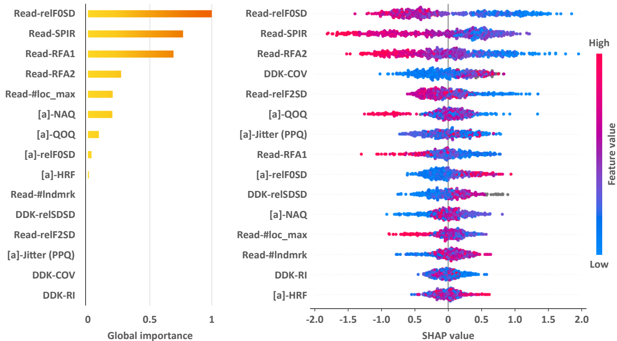
Figure 5: Global normalized combination of importance coefficients of robust features ( left ) and description of the model trained by robust features of all languages together using SHAP values ( right ) (features ordered from the highest absolute SHAP value, negative values indicate a higher probability for the classification to HC and positive values to patients with PD).
