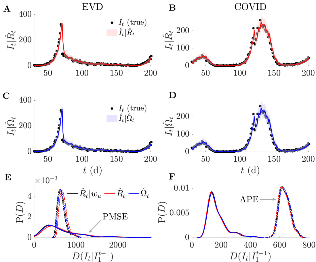
383 384 Figure 5: One-step-ahead prediction accuracy and model mismatch. We simulate 200 385 replicates of the epidemics from Figure 3 , which involve non-stationary changes to EVD and 386 COVID-19 generation times. We use estimates of effective, R , and angular, \Omega , reproduction 387 numbers to produce successive one-step-ahead predictions and assess their accuracy to the 388 simulated (true) incidence. Panels A-D provide a representative example of a single simulated 389 epidemic (true incidence shown as black dots) and the R and \Omega one-step ahead predictions 390 (red and blue respectively with 95% credible intervals). In panels E-F we formally compute 391 accuracy using distance metrics, D , based on accumulated prediction errors (APE, dashed) 392 and prediction mean square errors (PMSE, solid) for all 200 replicates from R , \Omega and R given 393 knowledge of the generation time changes i.e., R|w . We obtain distributions of D by applying 394 kernel smoothing. We find negligible differences in predictive power from all approaches.
