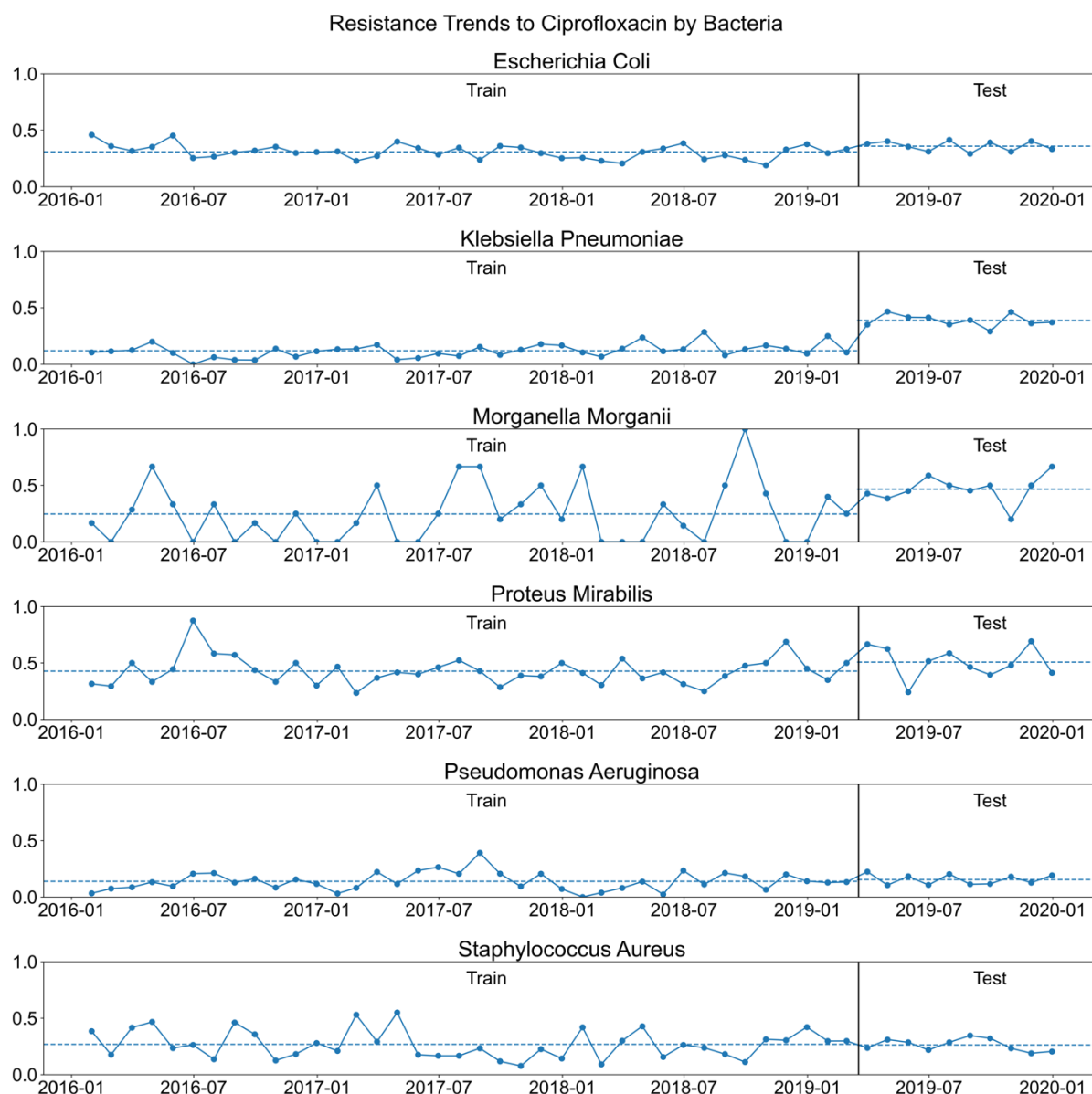
Figure 1: Ciprofloxacin resistance time-trends stratified by bacterial species. Points connected by solid lines are the average monthly ciprofloxacin resistance frequencies. The dotted horizontal lines represent the average resistance in the training and test sets, which are separated by the black vertical lines.
