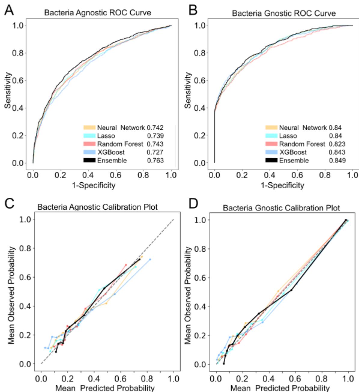
Figure 2: ROC curves (A, B) and calibration plots (C, D) for bacteria-agnostic and bacteria-gnostic datasets, respectively. ROC-AUC results of each model, on the test set, are presented within A and B. The colors represent different algorithms, where the black bold lines are the results of the ensemble model. Data points presented on the calibration plots are aggregated by deciles of predicted probability.
