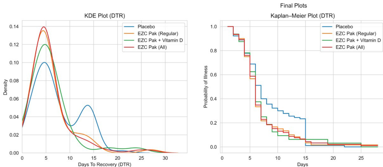
Figure 3. KDE and KM Plot for DTR Score.
