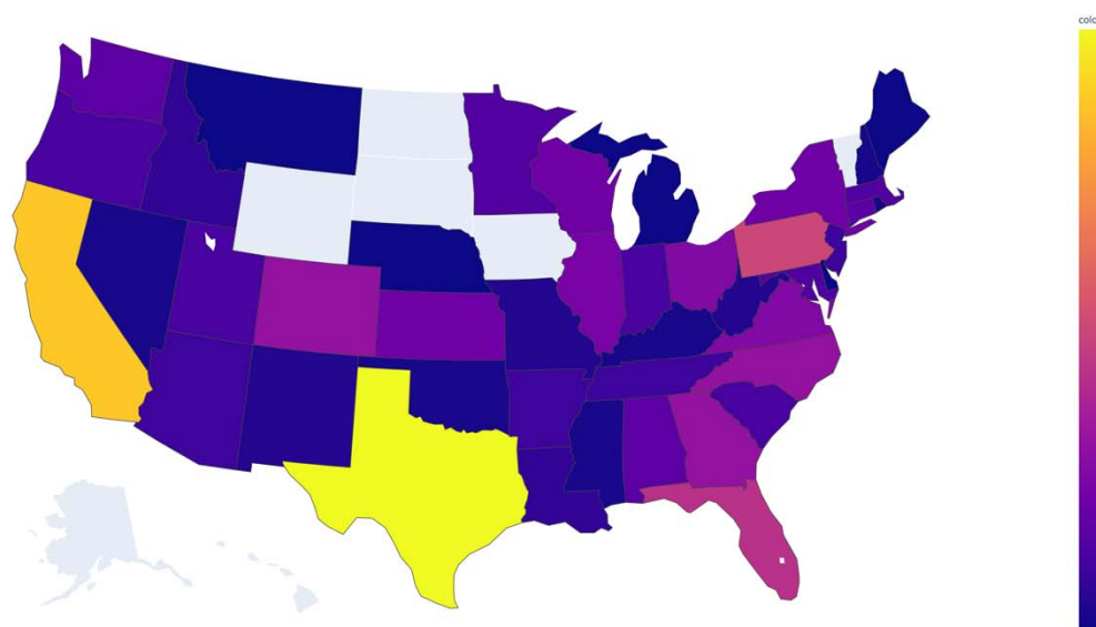
Figure 2. Choropleth Map of Geographic Distribution of Study Participants
