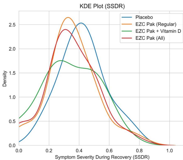
Figure 4. KDE Plot for SSSR Score
