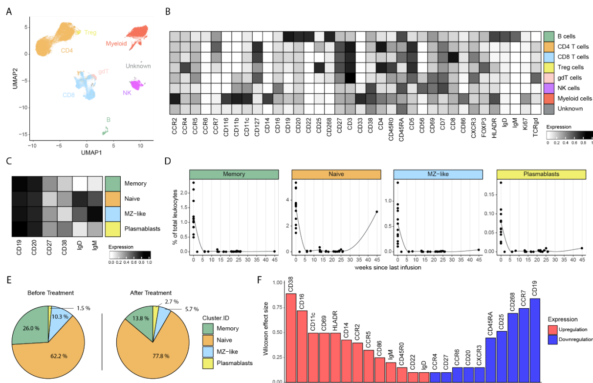
95 96 Fig. 1. BCDTs deplete B cells efficiently and alter the B cell phenotype after reconstitution. (A) UMAP of 52,500 97 cells randomly sampled from the combined dataset. The number of sampled cells was constant across samples. Color 98 code indicates the main clusters generated through clustering and manual annotation. (B) Heatmap showing the 99 median marker expression across the identified main clusters. (C) Heatmap shows the median marker expression 100 across the identified B cell sub-clusters. (D) Frequency of B cell subsets among total cells across time after infusion. 101 Points represent individual samples. The line represents the conditional mean of B cell subset frequency. (E) Pie chart 102 showing the composition of distinct subsets within the B cell compartment before (left) and after (right) treatment.
