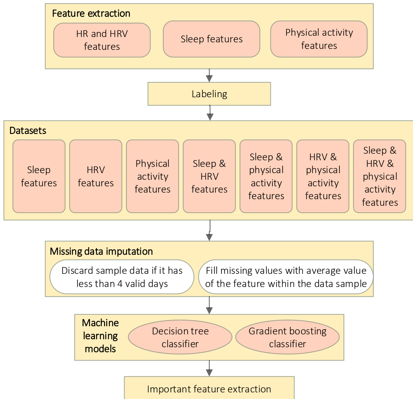
Fig 1. Machine learning pipeline
