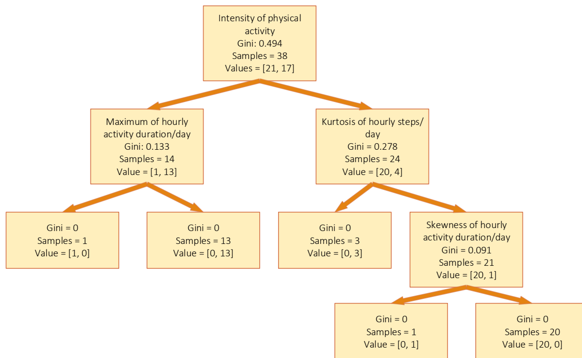
Fig 2. Features used in decision tree model for physical activity datasets
