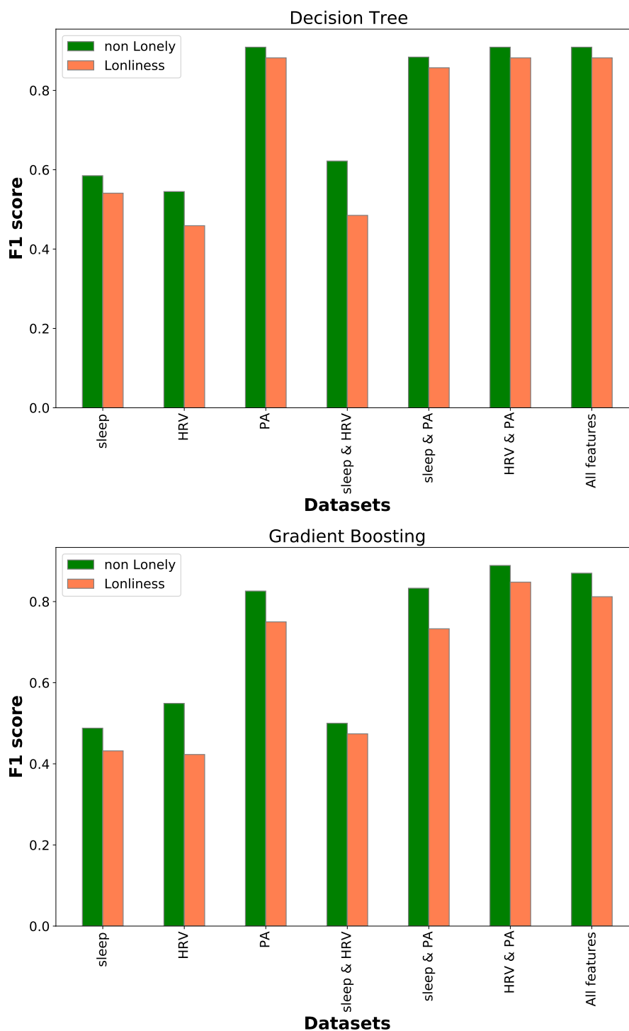
Fig 3. Classification results for different datasets
