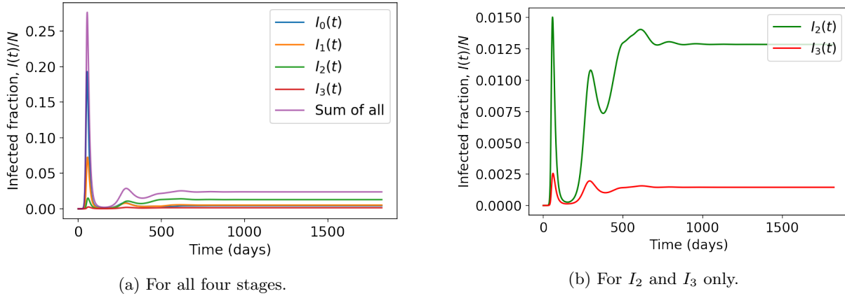
Figure 4: The change of infected fraction over time
