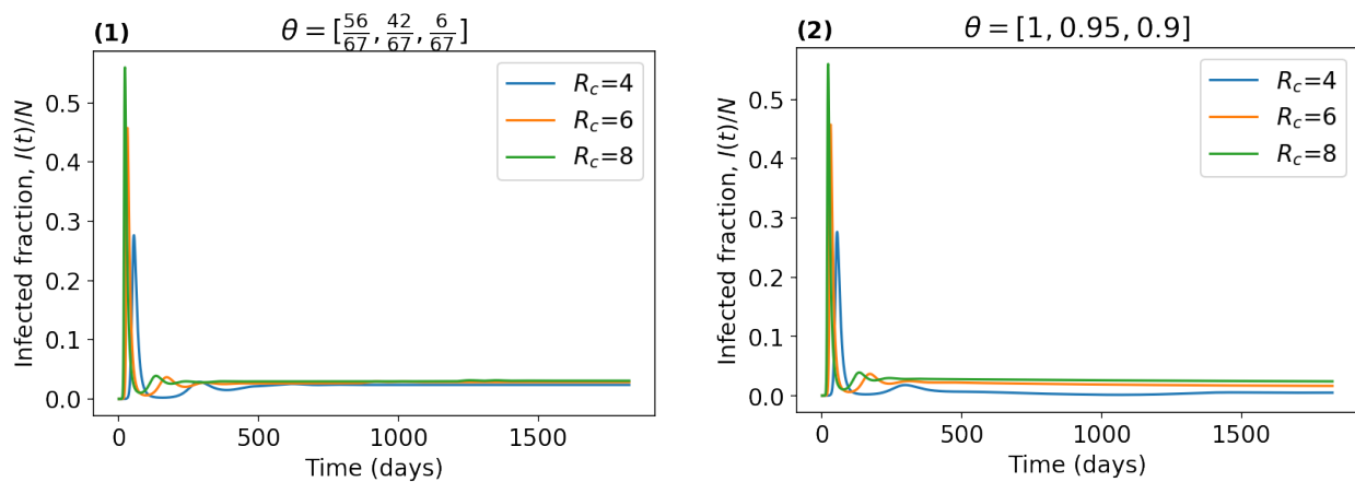
Figure 11: Changes in infected fraction \frac{I(t)}{N} for different R_c , and values used for other parameters are shown in Table 1.
