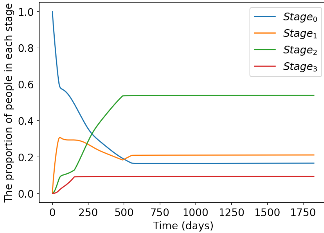
Figure 2: The proportion of people in each stage over time.
