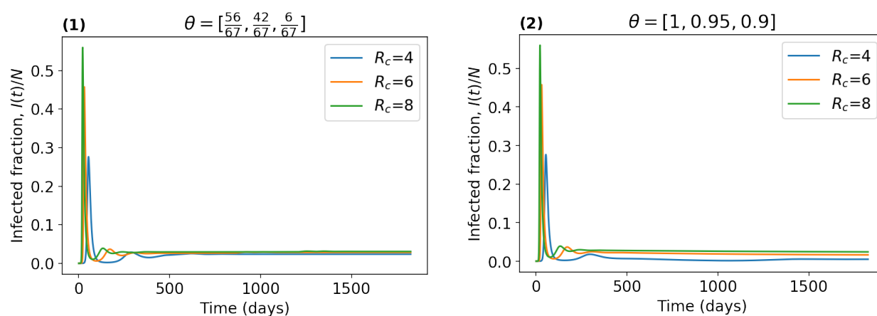
Figure 11: Changes in infected fraction \frac{I(t)}{N} for different R_c , and values used for other parameters are shown in Table 1.
