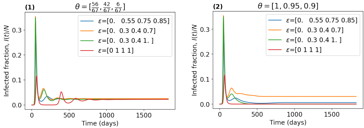
Figure 8: Changes in infected fraction \frac{I(t)}{N} for different \epsilon , and values used for other parameters are shown in Table 1.
