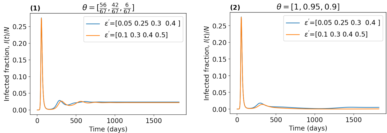
Figure 9: Changes in infected fraction \frac{I(t)}{N} for different \epsilon' , and values used for other parameters are shown in Table 1.
