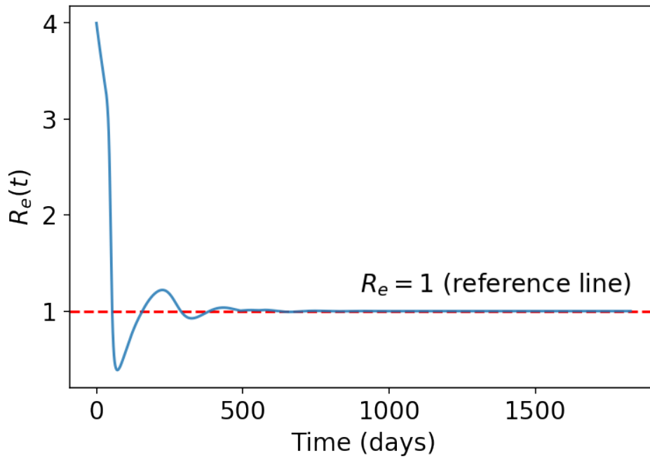
Figure 5: The change of R_e(t) .
