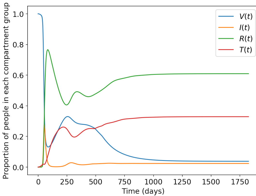
Figure 3: The proportion of people in each category of compartment over time.
