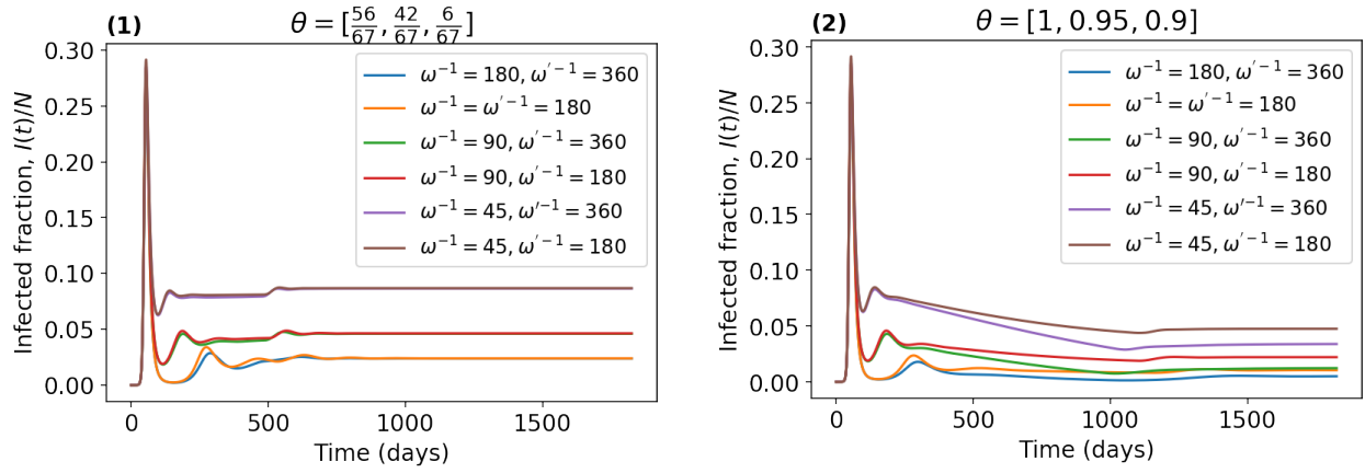
Figure 7: Changes in infected fraction \frac{I(t)}{N} for different \omega^{-1} and \omega'^{-1} , and values used for other parameters are shown in Table 1.
