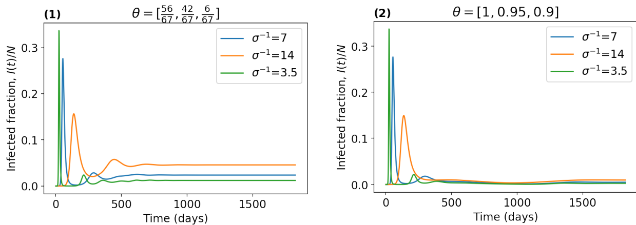
Figure 6: Changes in infected fraction \frac{I(t)}{N} for different \sigma^{-1} , and values used for other parameters are shown in Table 1.
