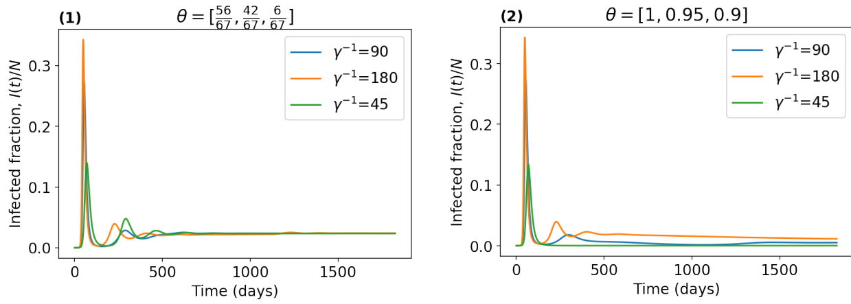
Figure 10: Changes in infected fraction \frac{I(t)}{N} for different \gamma^{-1} , and values used for other parameters are shown in Table 1.
