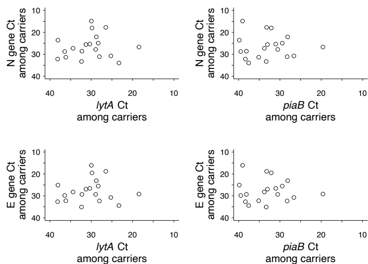
Figure S2: Correlation of qPCR C_T value for SARS-CoV-2 and pneumococcal gene targets in saliva samples. Panels illustrate C_T values for the SARS-CoV-2 nucleocapsid (N; top panels) and structural envelope protein (E; bottom panels) genes against C_T values for the pneumococcal lytA (left panels) and piaB (right panels) genes. Data are subset to individuals found to be infected with SARS-CoV-2 and to carry pneumococci.
