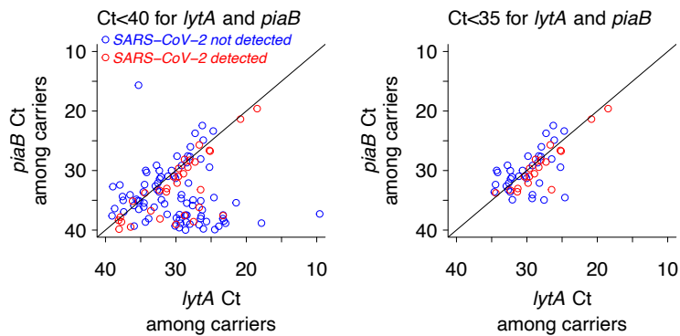
Figure S1: Correlation between lytA and piaB C_T values among pneumococcal carriers. Panels illustrate C_T values for all individuals found to carry pneumococci (based on C_T for both lytA and piaB ; left) and for individuals with C_T values below 35 for both lytA and piaB (right).
