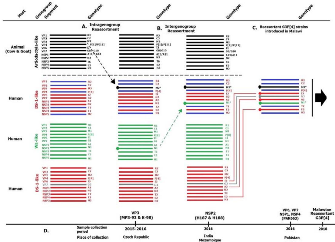
Figure 5. Reconstruction of the sequence of reassortment events that potentially lead to the emergence of the reassortant G3P[4] strains that were detected in Malawi. The reassortment events were hypothesised based on the genetic relationships between the genome segments of the reassortant DS-1-like G3P[4] rotaviruses that were detected in Malawi and those available in the NCBI Genbank to date. (A) The reassortant DS-1-like G3P[4] rotavirus strains that were detected in Malawi likely acquired their VP1, VP2, VP4, NSP1 and NSP5 genome segments from human DS-1-like rotaviruses and their VP3 from artiodactyl rotaviruses that circulated in countries where circulating rotaviruses have not been sequenced yet, or if done, their full-length genome sequences have not yet been deposited to the NCBI Genbank. (B) Both inter genogroup and intragenogroup reassortment events between Wa and DS-1-like rotaviruses were likely taking place from these unsampled regions, of which various progeny rotavirus populations were possibly generated. Reassortant DS-1-like strains that acquired their NSP2 through intergenogroup reassortment from Wa-like strains, which shared closest nucleotide similarity with rotaviruses that circulated in countries like Czech Republic between 2015 and 2016. (C) Various evolutionary events likely took place between the reassortant DS-1-like rotaviruses, DS-1-like G3P[4] and Wa-like G3P[8] rotaviruses that circulated in regions like Pakistan between 2014 – 2016, and in other unsampled regions that potentially led to various progeny rotavirus populations. One of the resultant progeny populations could be the reassortant DS-1-like G3P[4] strains from (B) that acquired NSP1, NSP4, VP6 and VP7 from the DS-1-like G3P[4] strains that were circulating in regions like Pakistan through complex reassortment events. The resultant reassortant DS-1-like G3P[4] rotaviruses were the ones that were exported to Malawi and caused diarrhoea disease in children that were hospitalised at Queen Elizabeth Central Hospital in Blantyre, Malawi from 2018, or circulated in unsampled regions. (D) The period and country where the closest related strains to the genome segments of the reassortant DS-1-like G3P[4] were detected. The horizontal line represents the 11 rotavirus genome segments.
