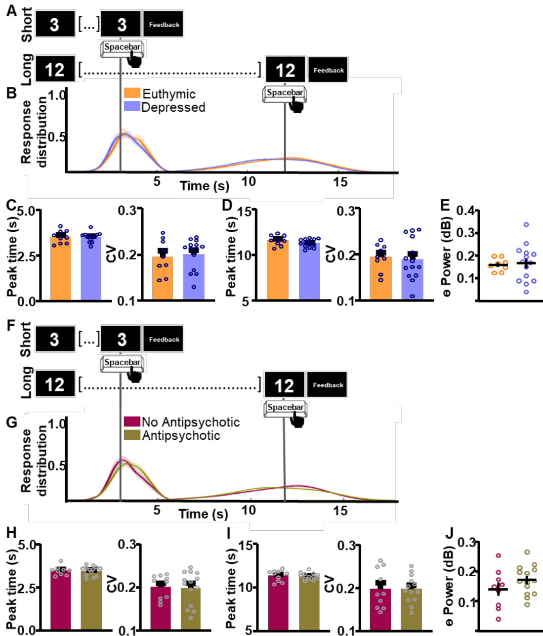
568 Figure 5. Interval timing performance and frontal theta power do not differ as a function 569 of mood or medication status. A. To assess task-wide differences in oscillatory activity data 570 from the whole interval-timing task were analyzed. B. Response distribution for individuals with 571 bipolar disorder who were either euthymic or depressed at the time of data collection. C-D. 572 Groups do not differ in time estimation for the short [ C ] or the long [ D ] intervals. E. Frontal
