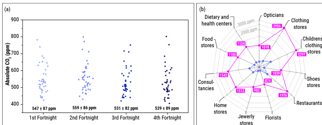
307 308 Figure 5. (a) Mean of CO 2 value (inbox) of all businesses based on the fortnight and (b) mean of CO 2 309 and maximum measurement depending on the type of business where the mean value (blue) and 310 the maximum values (pink label) are shown.
