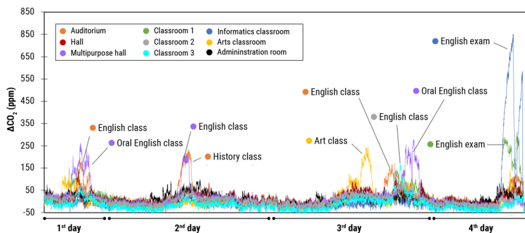
197 Figure 2. Increment of CO 2 values recorded in the diagnostic period.
