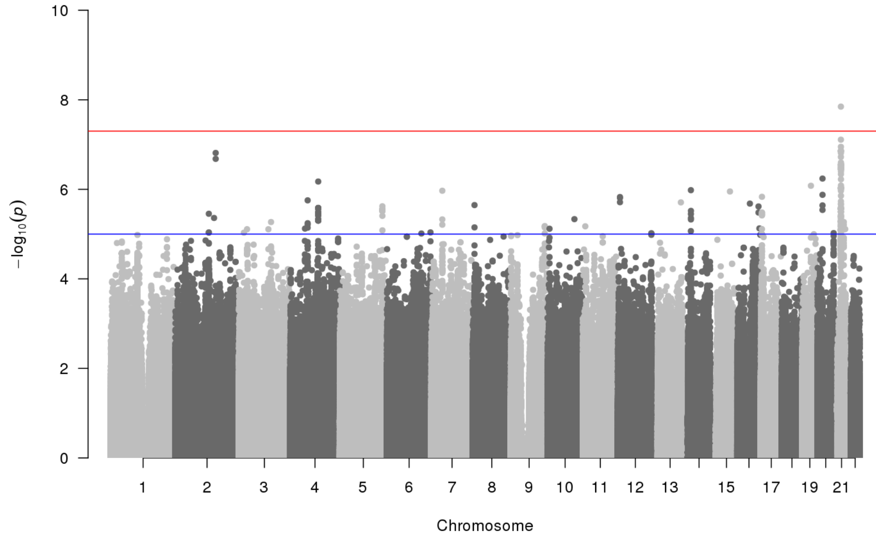
Figure 4: Manhattan plots from the GWAS results of NETs conducted with Compound Poisson-Gamma model
