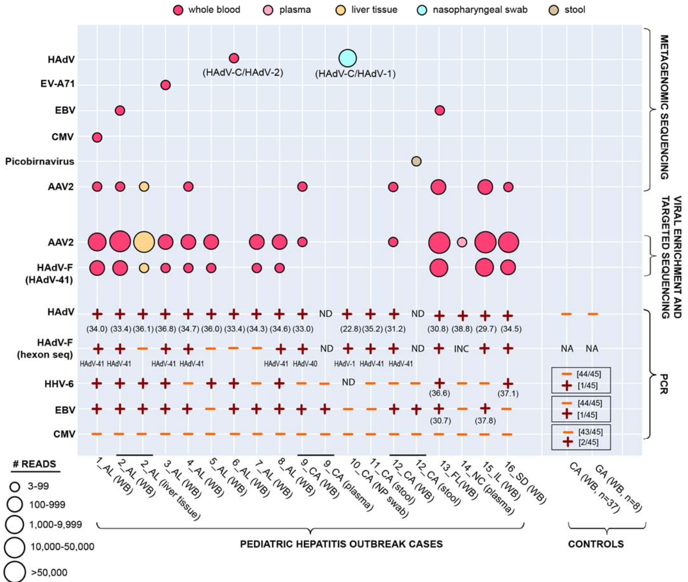
Figure 2. Overview of next-generation sequencing and molecular-based testing performed on cases and controls. Each circle represents a sequenced sample with at least 3 non-overlapping reads 20 aligning to a viral sequence in the National Center for Biotechnology Information (NCBI) database detected by metagenomic and targeted or virally enriched sequencing. The circles are color-coded based on the sample type and size-scaled based on viral read counts. PCR positive and negative results are denoted by plus and
