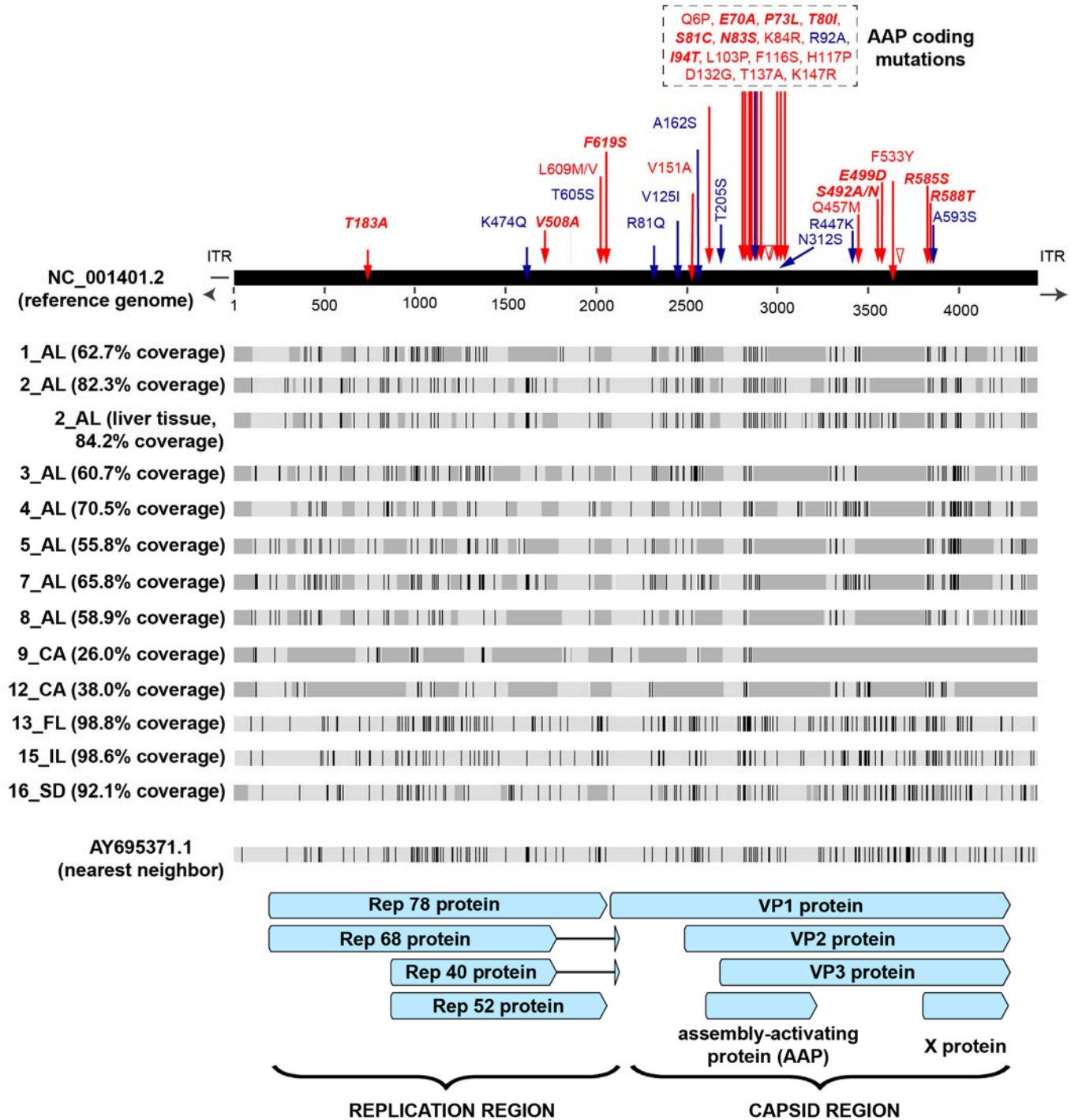
13 14 Figure 5. Adeno-associated virus 2 variant analysis. Multiple sequence alignment of adeno-associated 15 virus genomes recovered from the acute hepatitis cases. Nucleotide mismatches are represented by black- 16 colored vertical lines, while areas of missing coverage are represented by gray rectangles. Amino acid variants 17 with respect to the reference genome (NC_001401.2) are denoted in blue and red arrows; red arrows indicate
