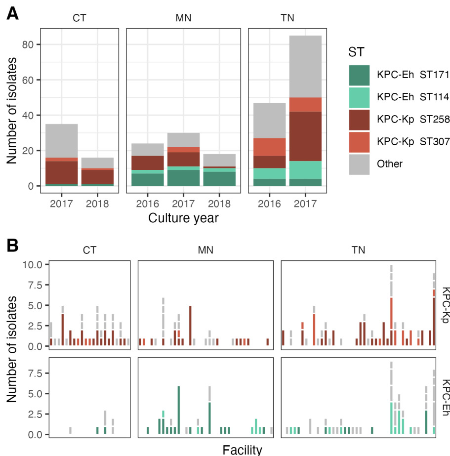
905 906 Figure S1: Distribution of species and sequence types of sequenced isolates from each state. 907 (A) Across time. (B) Across healthcare facilities with at least one identified CRE with blaKPC . 908 X axis shows facilities. Grey is any other ST of the species corresponding to that faceted plot. 909 Notes: The MuGSI catchment area for MN is Hennepin and Ramsey counties. Four counties in 910 the Memphis-Delta Emergency Medical Services (EMS) and 8 in Northeastern TN were 911 excluded due to extensive healthcare utilization across state lines; the MuGSI catchment area is 912 TN EMS Region 5, an 8-county region encompassing the metropolitan Nashville area, of TN. 913 CT=Connecticut; MN=Minnesota; TN=Tennessee; ST=sequence type; Eh= E. hormaechei ; 914 Kp= K. pneumoniae . 915
