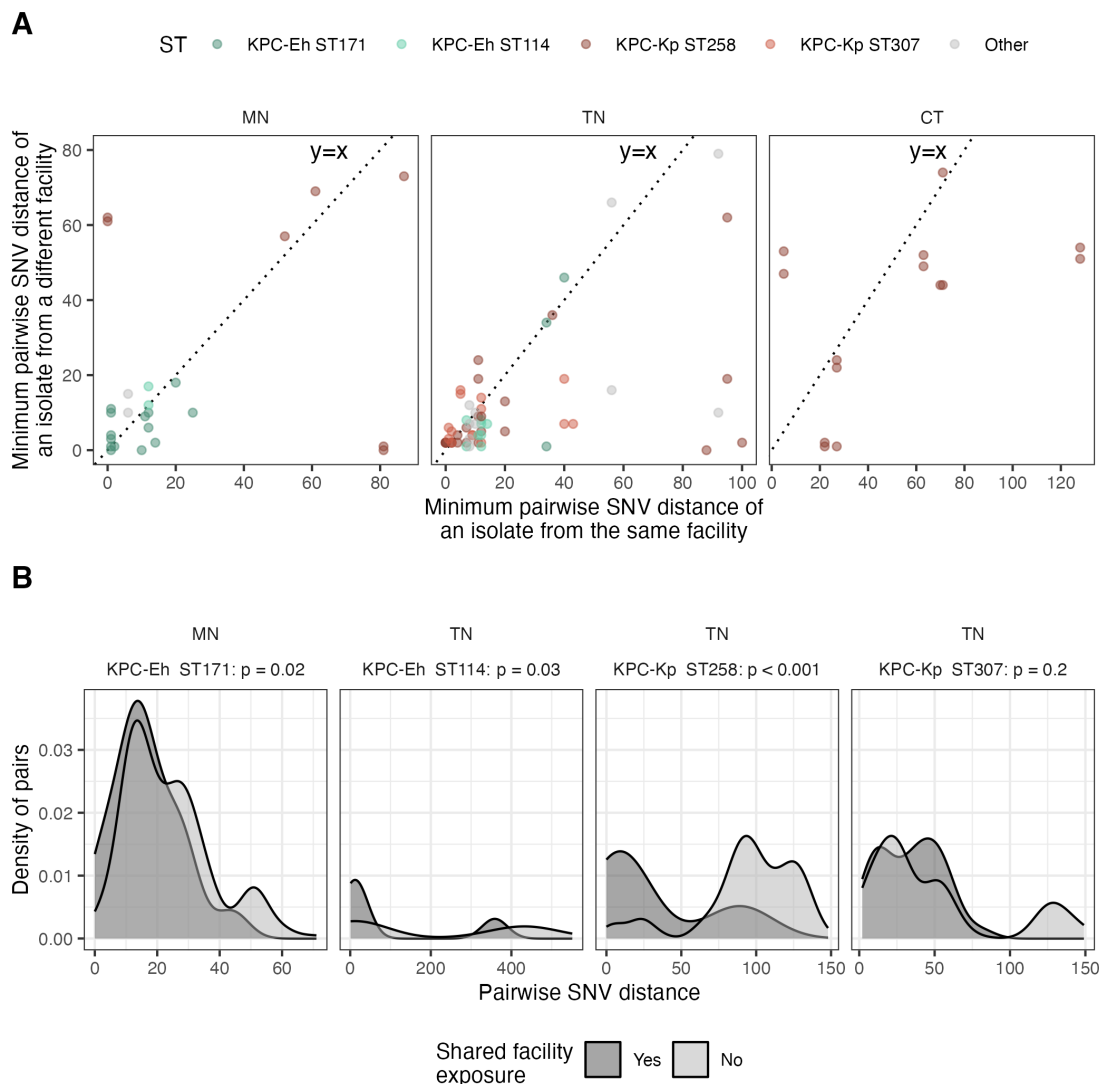
601 602 Figure 2: Small pairwise single nucleotide variant (SNV) distances suggest 603 that local transmission was captured. (A) For each isolate with at least one intra-facility isolate 604 pair and at least one inter-facility isolate pair, pairwise SNV distance of the most closely related 605 intra-facility compared to the most closely related inter-facility isolate. (B) Pairwise SNV 606 distance of inter-facility isolate pairs from patients with a shared facility exposure compared to 607 those not linked by a shared facility exposure. A shared facility exposure is when individuals 608 with isolates from different facilities both spent time in the same facility at some point in the last 609 year. Only STs with >10 isolate pairs with a pairwise SNV distance of \leq 15 are shown. One-sided
