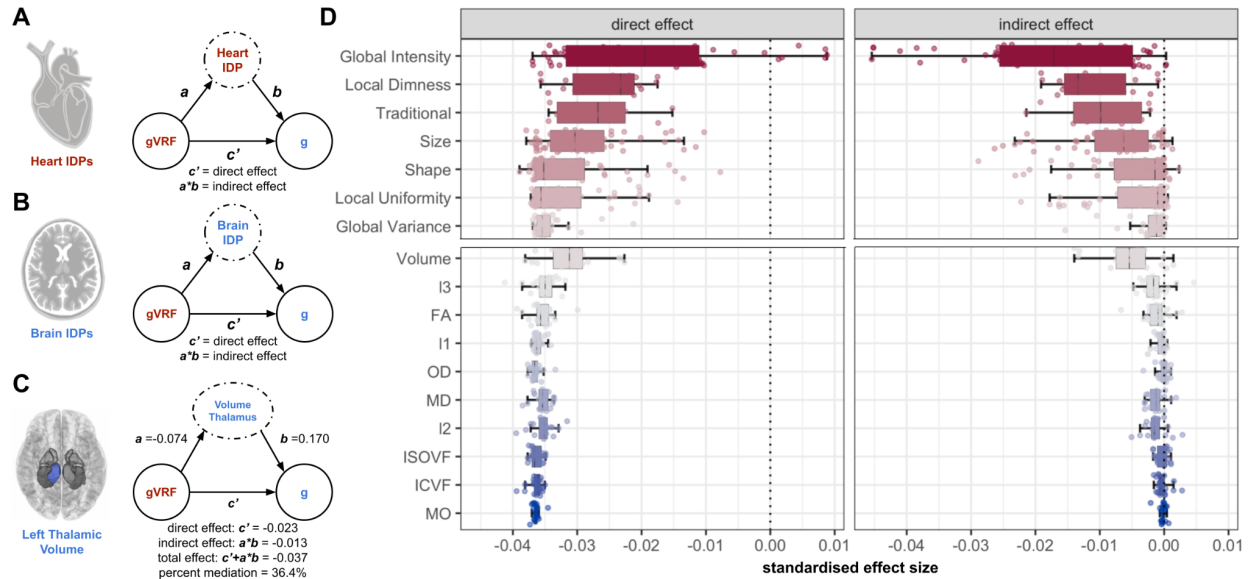
Figure 6: Individual Feature Single Mediation Modelling
