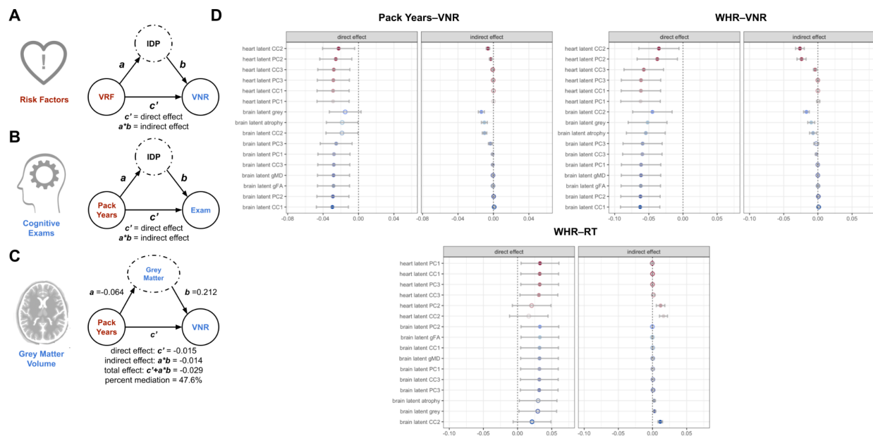
Figure 5: Latent Single Mediation Modelling of VRF-Cognitive Pairs
