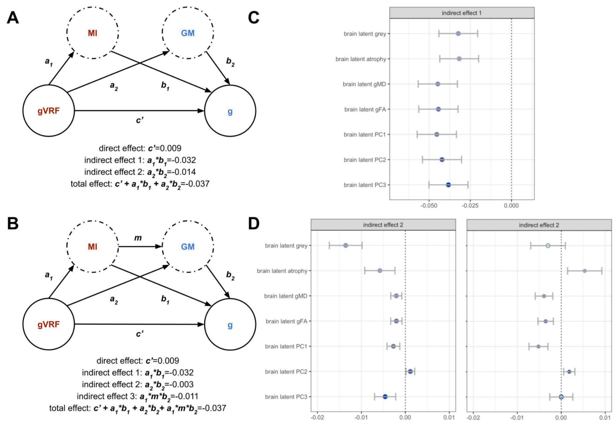
Figure 4: Latent Multiple Mediation Modelling
