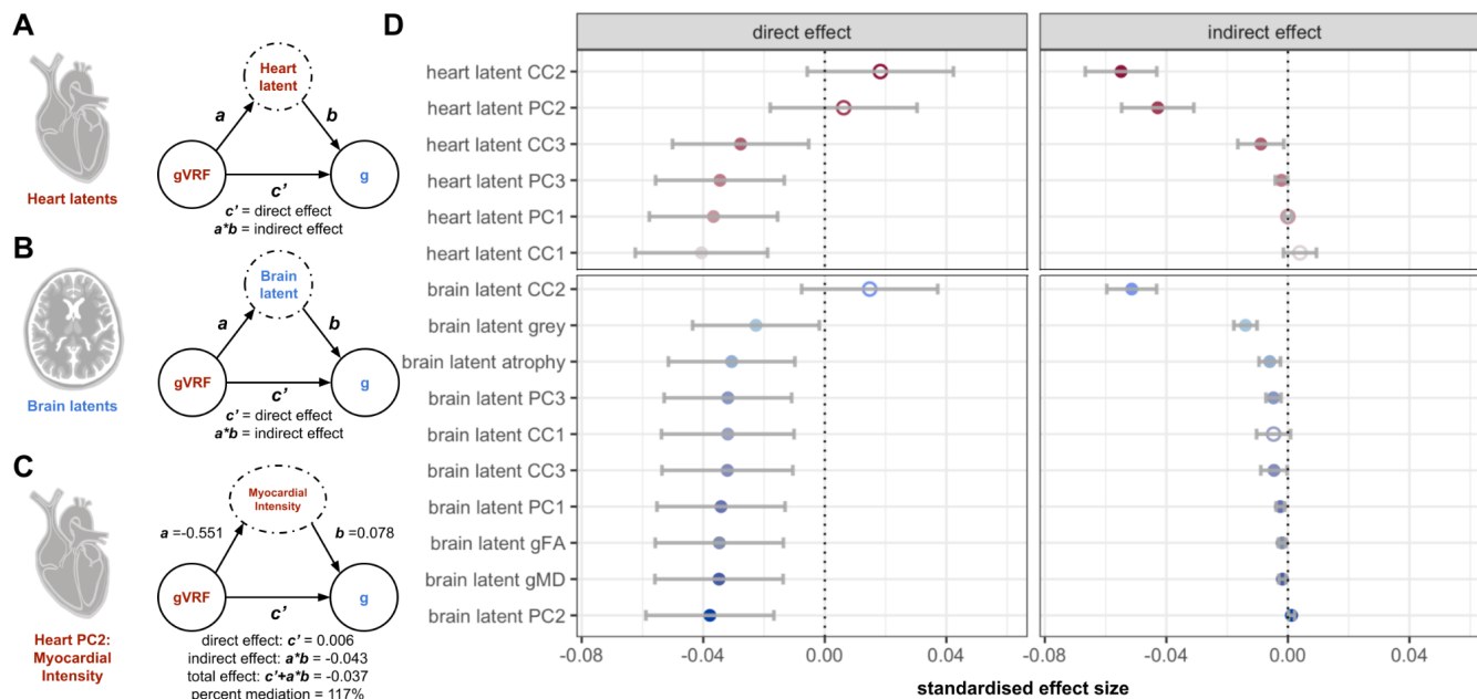
Figure 3: Latent Single Mediation Modelling
