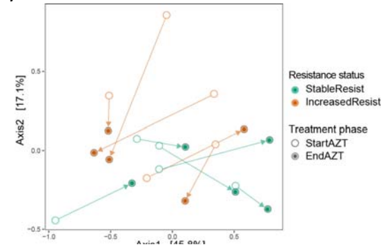
Figure 7. Relationship between the difference in ARG carriage during AZT treatment, bacterial load and the 15 dominant genera of the LRT microbiota. (a) qPCR determination of bacterial load showing lower levels in patients with increased resistance. (b and c) Double PCoA showing the influence of Prevotella_7 abundance in the compositional changes occurring during AZT treatment in patients with stable resistance, respectively Streptococcus abundance in patients with increased resistance. In panel c, the arrows link LRT samples collected from a single patient at the start and end of AZT treatment.
