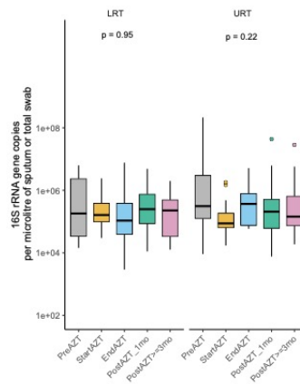
Figure 2. qPCR determination of 16S rRNA gene copy number per microlitre of sputum or total OPS samples showing no variation in bacterial load during the different phases of the study. Abbreviations: qPCR = quantitative polymerase chain reaction; OPS = oropharyngeal swab
