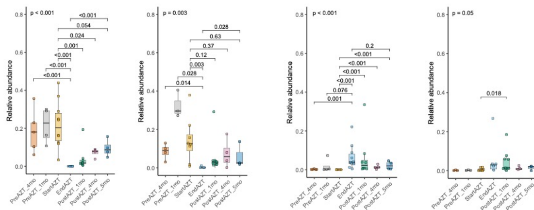
Figure 5. Longitudinal changes in the relative abundance of bacteria cleared (a) or acquired (b) in the LRT during AZT treatment, showing different magnitudes of change in relative abundance between cleared and acquired bacteria, and similar kinetics between LRT and URT. Abbreviations: LRT = lower respiratory tract; AZT = azithromycin; URT = upper respiratory tract
