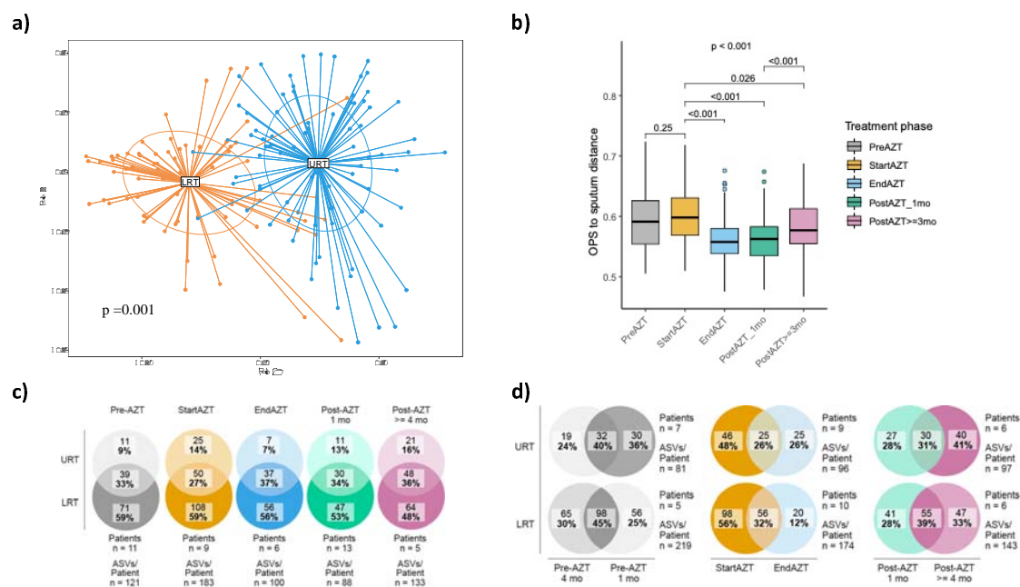
Figure 4. AZT treatment reduces dissimilarity between LRT and URT microbiota. (a) PCoA based on unweighted UniFrac distance showing an overall difference in bacterial community composition between URT and LRT. (b) Aitchison distance showing a decrease in dissimilarity between URT and LRT microbiota between the start and end of treatment. For each treatment phase, Aitchison distance was calculated between each OPS sample and the centroid obtained from the corresponding set of sputum samples. (c) Venn diagrams of the numbers and proportions of ASVs represented in either the LRT or URT alone, or in both sites, showing that the decrease in dissimilarity between the LRT and URT microbiota during treatment was in part driven by a decrease in the proportion of ASVs present in the LRT alone. (d) Venn diagrams of the numbers and proportions of ASVs represented either at the start, at the end or retained over a 3-month time window, showing a decrease in ASV turnover after AZT treatment in both LRT and URT.
