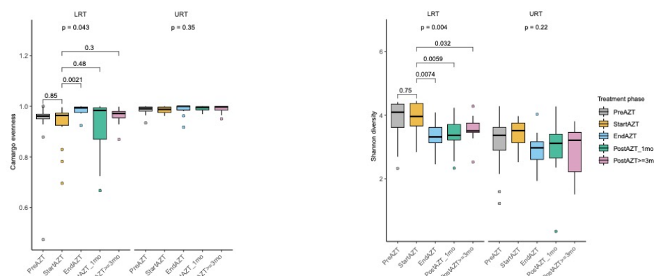
Figure 3. Decrease in community diversity after AZT treatment. (a to d) Alpha diversity metrics showing a decrease in Chao1 richness (a) and Faith's diversity (b) during AZT treatment in LRT and URT, an increase in Camargo evenness in LRT (c), and a decrease in Shannon diversity in LRT (d).
