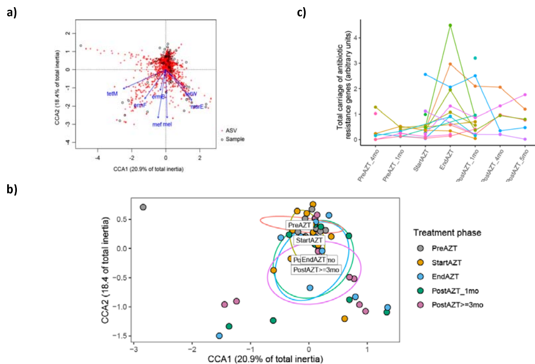
Figure 6. Acquisition of ARG during AZT treatment in LRT. (a and b) Canonical correlation analysis showing that ARG carriage was limited to a minority of sputum samples (circles) and ASVs (crosses) (a), and stratification by treatment phase showing that almost all samples with ARG were taken at the end of AZT treatment or later (b). (c) Within-patient monitoring of the cumulative sum of normalised copy numbers of the full set of ARG genes, focusing on patients with more than one sputum sample available, showing the increase in ARG carriage after the start of AZT treatment.
