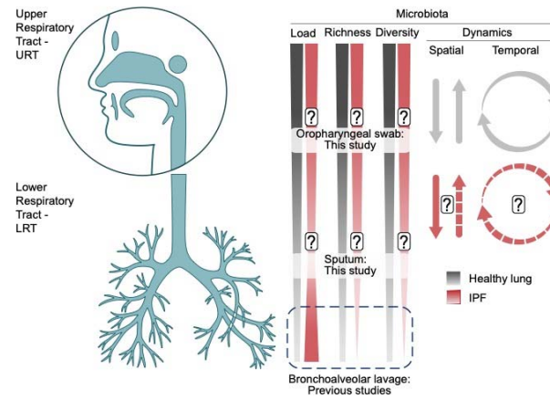
Figure 1. In health, the LRT microbiota is a community of transiently present microorganisms originating from the URT, whereas in IPF the LRT microbiota is a thriving community with a higher bacterial load and a decreased community diversity. The spatial dynamics between the URT and LRT microbiota in IPF, their turnover rates, and how these are affected by AZT remains unknown. Abbreviations: LRT = lower respiratory tract; URT = upper respiratory tract; IPF = idiopathic pulmonary fibrosis; AZT = azithromycin
