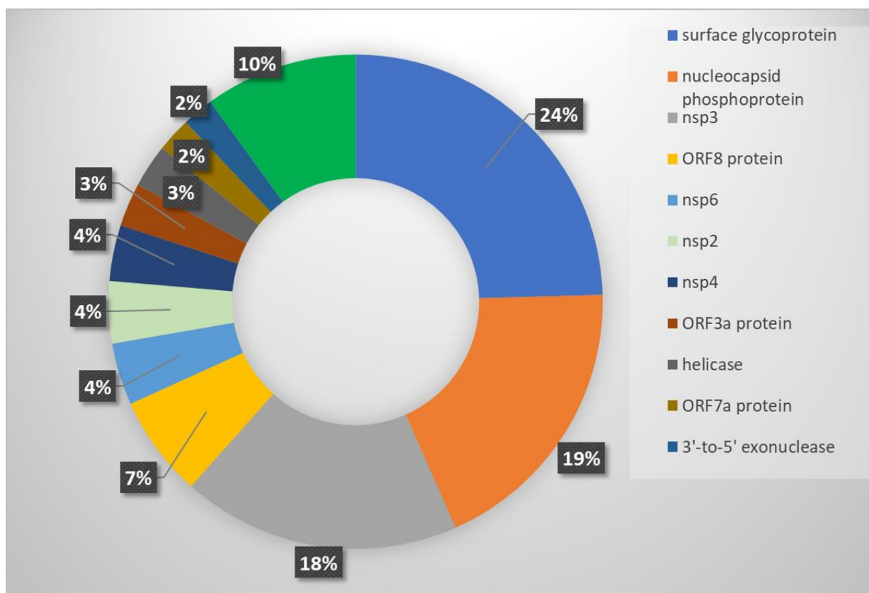
Figure 3. Distribution of major hotspot mutant genes in 405,461 global samples with complete SARS-CoV-2 genome sequences. Complete genomes sequences from National Center for Biotechnology Information (NCBI) database were analyzed for top mutant genes as of August 4 th , 2021, a total of 405,461 complete SARS-CoV-2 genomes from 88 countries were analyzed.
