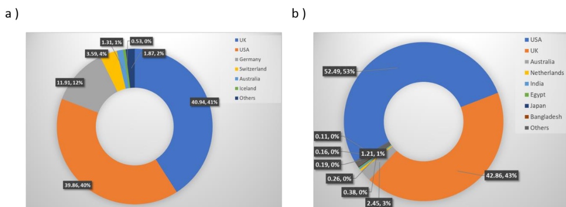
Figure 2. Global distribution of severe acute respiratory syndrome coronavirus 2 (SARS-CoV-2) genomes by sample collection locations from 101 countries. a) Distribution of 1,012,582 SARS-CoV-2 genomes (complete and partial genome sequence) by countries as of August 4 th , 2021. b) Global distribution of 405,461 complete SARS-CoV-2 genomes by region (from 88 countries).
