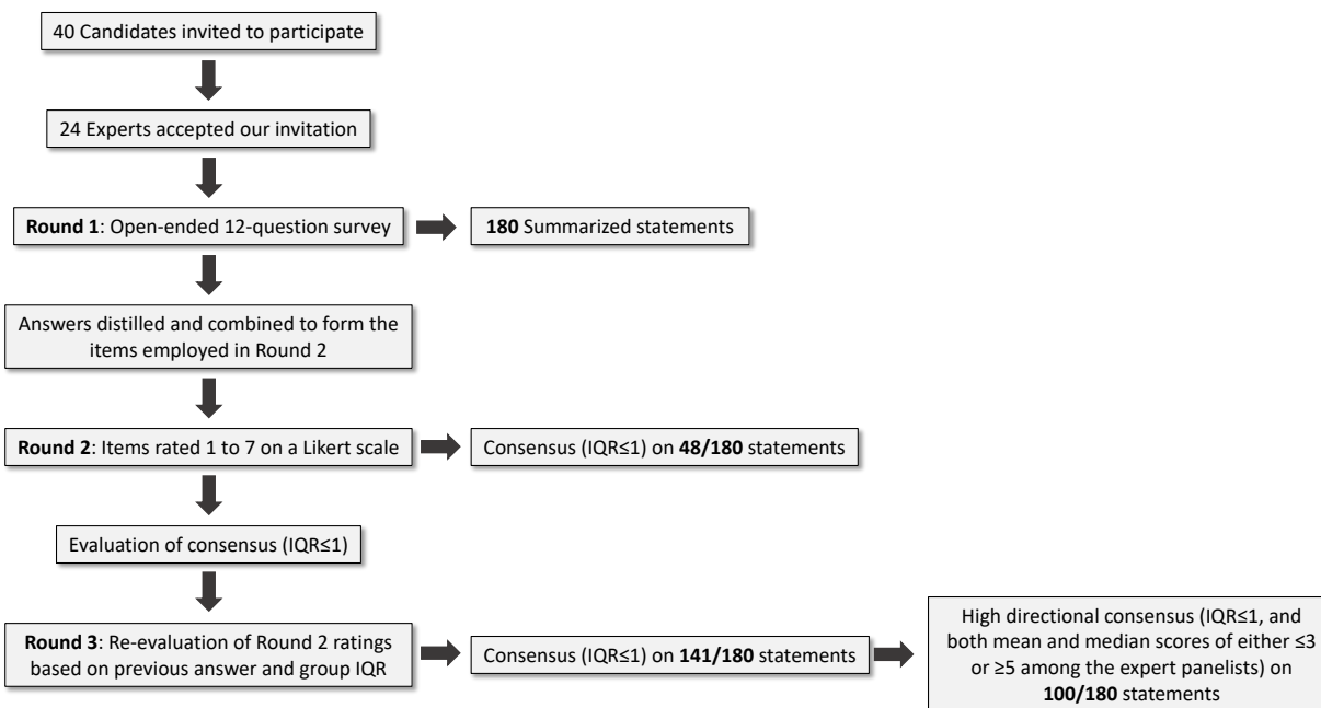
200 201 Figure 1. Flowchart illustrating the process of the present Delphi study 202
