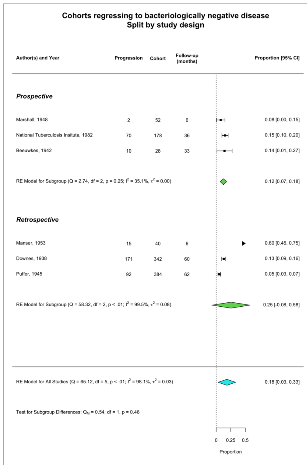
30 Figure 3b: participants entering cohorts with positive microbiology, transitioning to negative 31 microbiology: forest plot of the random effects meta-analysis of annualized rates (as described fully in 32 methods section) with proportion and 95% confidence intervals for subgroups, according to study design 33 34
