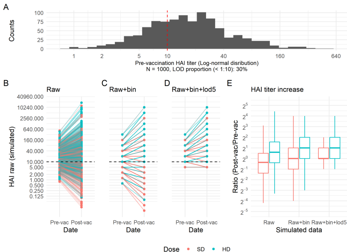
Figure 1: Simulated HAI titer and LOD. A, example of a simulated log-normal distributions with a total sample size equal to 1000 with about 30% values below LOD; B, the simulated raw data; C, the simulated raw+bin data (binning raw data into discrete integers); D, the simulated raw+bin+lod5 data, introducing the LOD issue (<1:10 coded as 1:5) into the simulated raw+bin data; E, HAI titer increase for both HD and SD vaccines using the three versions of simulated data.
