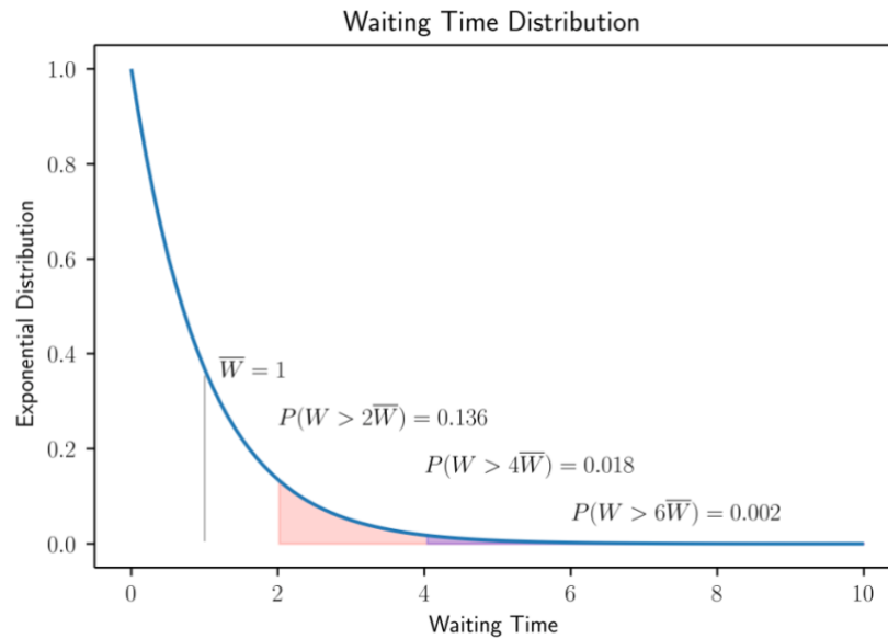
Figure 2. The probability distribution of waiting times for a stable queue.
