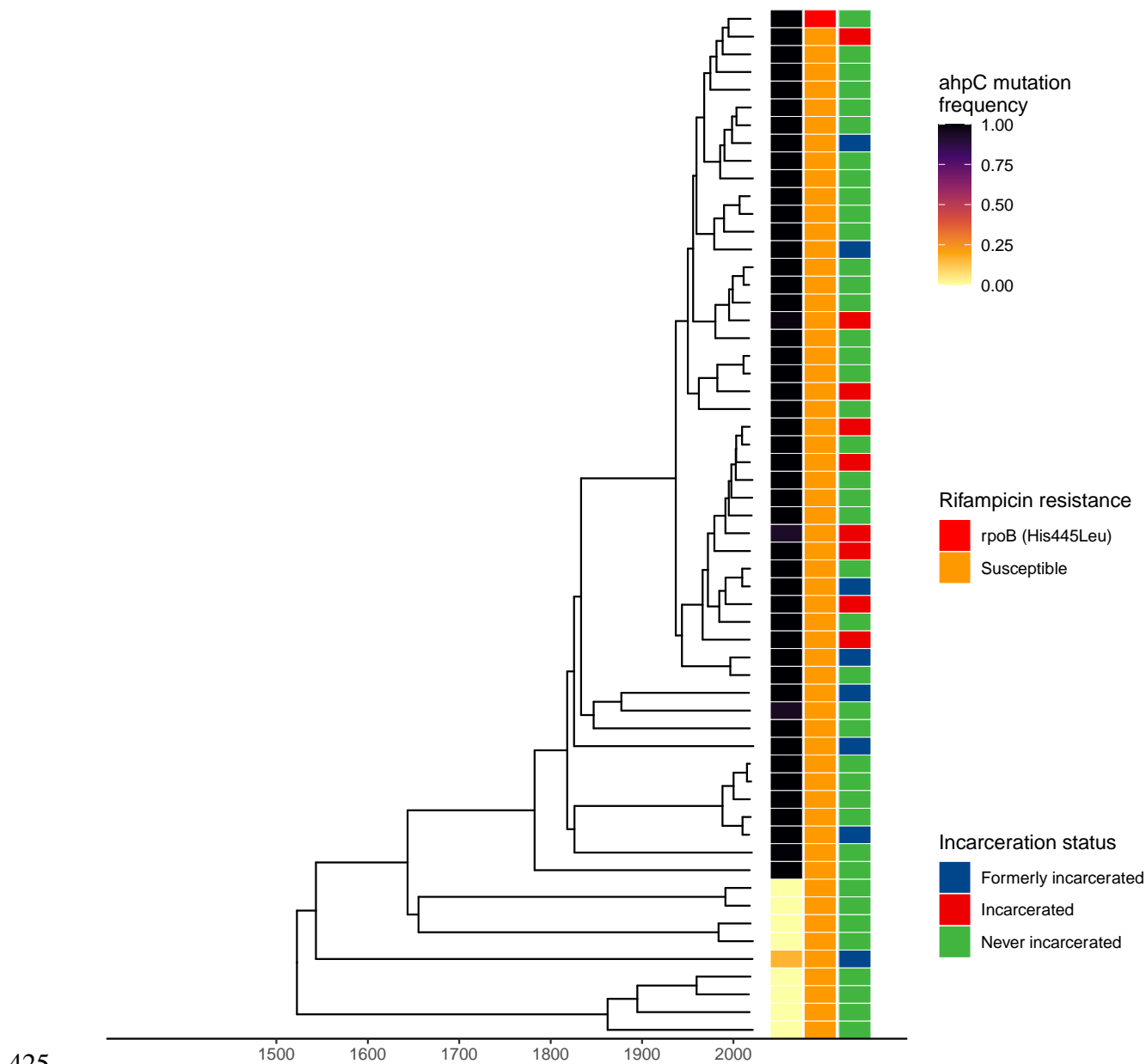
Figure 5. Emergence of a putative resistance-associated ahpC promoter mutation. Time-scaled Bayesian maximum clade credibility tree for 58 samples in sublineage 4.4.1.1. Branch lengths are in years and grey bars indicate 95% high posterior density estimates of node date. The heatmap to the right of the phylogeny indicates patient incarceration status at the time of TB notification, ahpC mutation frequency within an individual's infection, and the occurrence of a rifampicin resistance-conferring mutation ( rpoB His445Leu).
