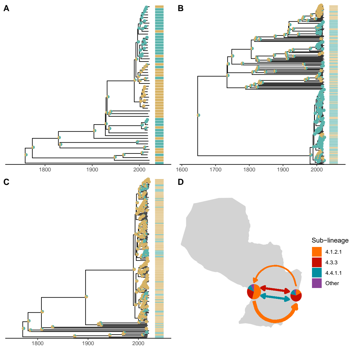
405 406 Figure 3. Frequent gene flow of M. tuberculosis connects Paraguay's major urban centers. (a-c) We 407 used discrete ancestral state reconstruction to reconstruct migration between the two cities for the three 408 dominant sub-lineages in our sample; lineages 4.1.2.1, 4.3.3, and 4.4.1.1. Bayesian maximum clade 409 credibility trees of samples in the three dominant sub-lineages with tip points colored by city of sampling 410 and pie charts at nodes indicating the inferred ancestral location. Branch lengths are in years and grey bars 411 indicate 95% high posterior density estimates of node date. (d) Map of Paraguay with pie charts 412 indicating the genomic diversity sampled in Asunción (at Paraguay's western border) and Ciudad del Este
