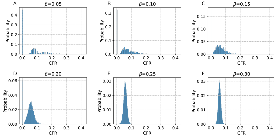
Figure 10: Final probability distribution for the case fatality ratio for different values of \beta . In each case 50,000 realisations were simulated with \mu_R^0 = 5 , \mu_R^1 = 6 , \mu_R^2 = 12 , \mu_R^3 = 4 , and \mu_D^0 = 5 , \mu_D^1 = 5 , \mu_D^2 = 5 , \mu_D^3 = 9 for the multistage sED. As before, the initial population size for these simulations is 1000. A phase shift from a multimodal distribution to a unimodal distribution can be observed when \mathcal{R}_0 = \mu_R^0 \beta (S(0)/T) > 1 , happening for \beta > 0.2 .
