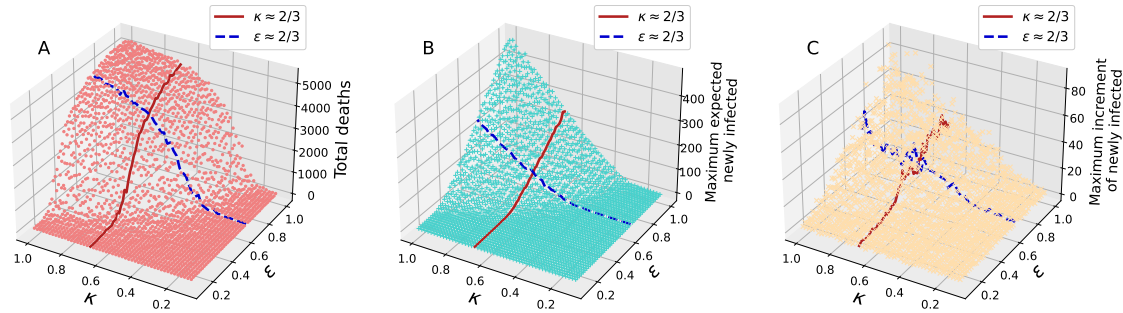
Figure 7: Quantities of interest that directly depend on I(t) , as a result of varying the exposure for susceptible and infected ( \epsilon and \kappa ) in the basic sED model. The solid line in red corresponds to the case \kappa = 2/3 , and the dashed line in blue corresponds to the case \epsilon = 2/3 . (A) Total deaths, (B) maximum expected value of the newly infected individuals, and (C) maximum increment of the newly infected individuals between t and t + h .
