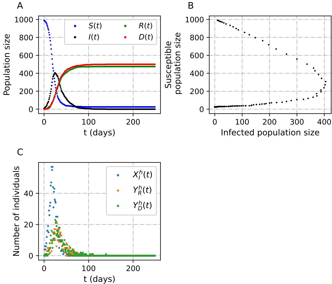
Figure 2: Dynamics and geometry of the sED model. (A) Epidemiological curves obtained with the sED model. (B) I - S phase plane. (C) Numbers of newly infected individuals, of people that recover, and of people that die over time. The parameters used in this simulations were \mu_R = 27 , and \mu_D = 24 . Other parameters can be found in table 1.
