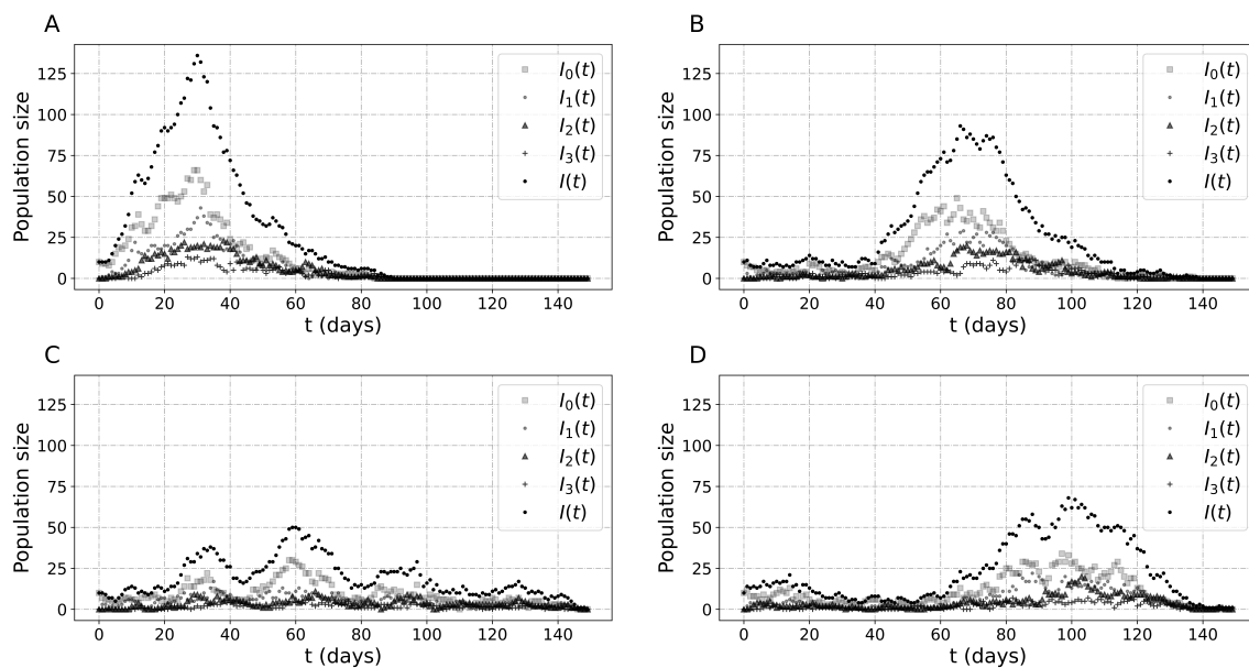
Figure 8: Different dynamics observed in the multistage sED. Realisations in all cases were simulated assuming the same total expected infection time with \mu_R^0 = 5 , \mu_R^1 = 6 , \mu_R^2 = 12 , \mu_R^3 = 4 , and \mu_D^0 = 5 , \mu_D^1 = 5 , \mu_D^2 = 5 , \mu_D^3 = 9 for the multistage sED. As before, the initial population size for these simulations is 1000.
