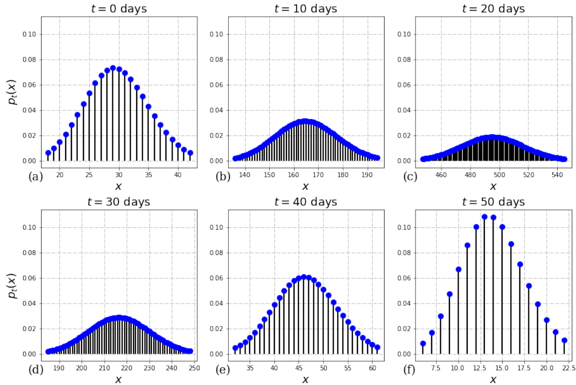
Figure 4: Example of the evolution of the probability mass function p_t(x) of new infections x in the basic sED model as a function of time t . The parameters used in the simulation were T_0 = 10,000 , \beta = 0.3 , \mu_R = 27 , \mu_D = 24 and h = 1 .
