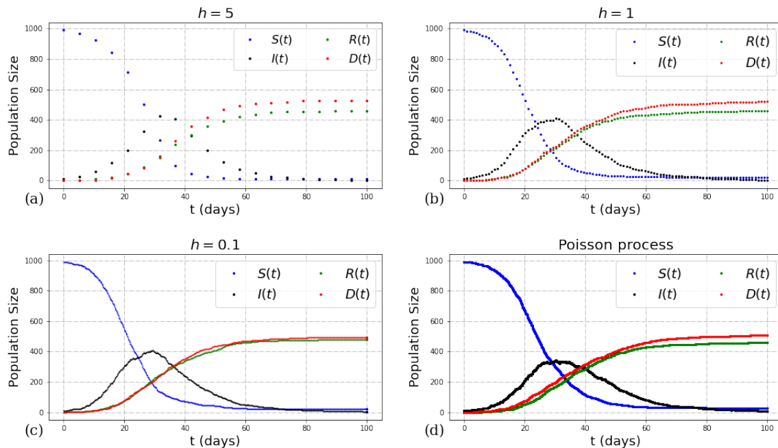
Figure 5: Realisations of the sED model dynamics for a decreasing step sizes ( h ) and the approximation of the model using the Poisson process. For this simulation \mu_R = 27 and \mu_D = 24 , and the other parameters can be found in Table 1.
