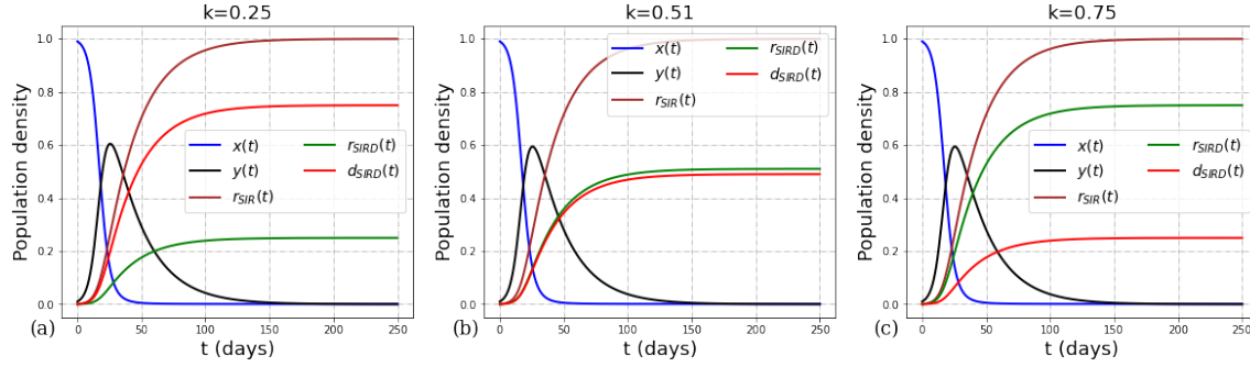
Figure 7: Systematic comparison between the dynamics of the SIR and SIRD models. The comparison was made assuming that \gamma = \gamma_d + \gamma_r with \gamma_d = k\gamma , and \gamma_r = (1 - k)\gamma and k \in \{0.25, 0.51, 0.75\} , with \gamma = 2/(27 + 24) .
