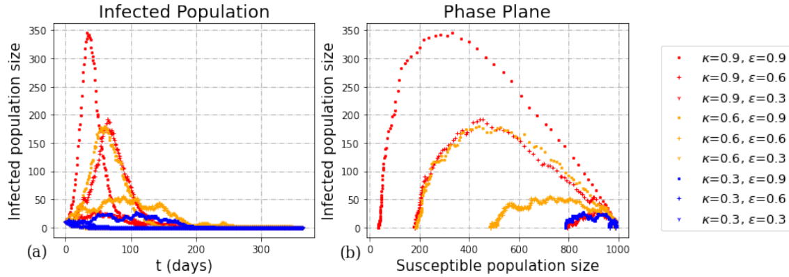
Figure 8: Infection processes varying the exposure for susceptible and infected ( \varepsilon and \kappa ). S - X^h phase plane for different values of p . Realisations were calculated using \mu_R = 27 , and \mu_D = 24 .
