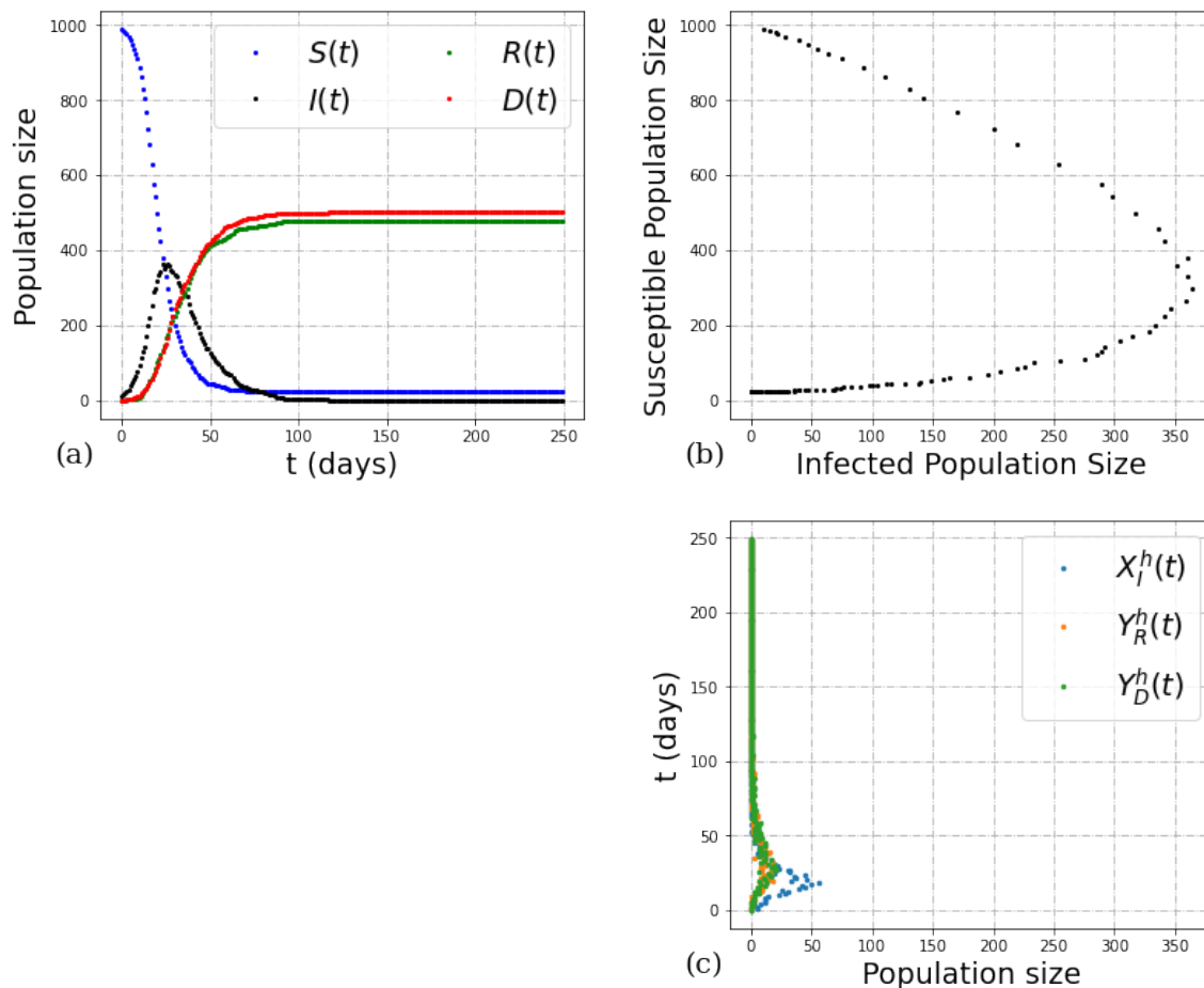
Figure 3: Dynamics and geometry of the sED model. The parameters used in this simulation were \mu_R = 27 , and \mu_D = 24 . Other parameters can be found in Table 1.
