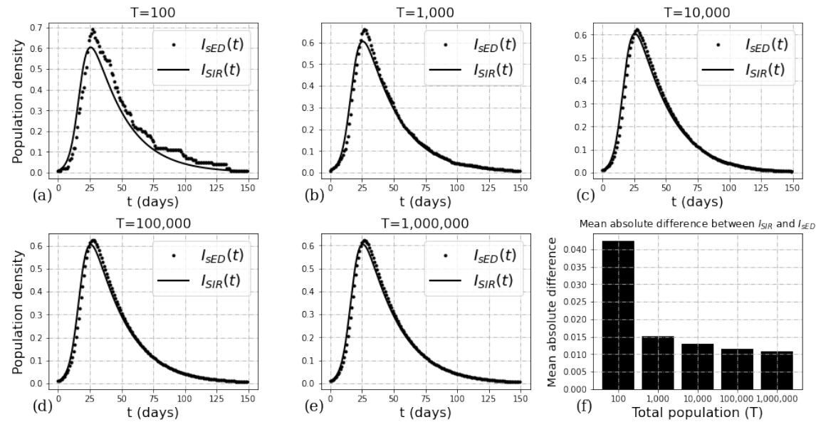
Figure 6: Density of infections for different population sizes of SIR vs sED dynamics obtained by replacing the sampling processes by their mean at each time step. The bars indicate the size of the difference between the total infected over time between the two models as a function of the population size. For these realisations, \mu_R = (27 + 24)/2 for the sED model without deaths, and \beta = 0.3 and \gamma = 2/(27 + 24) for the SIR model.
