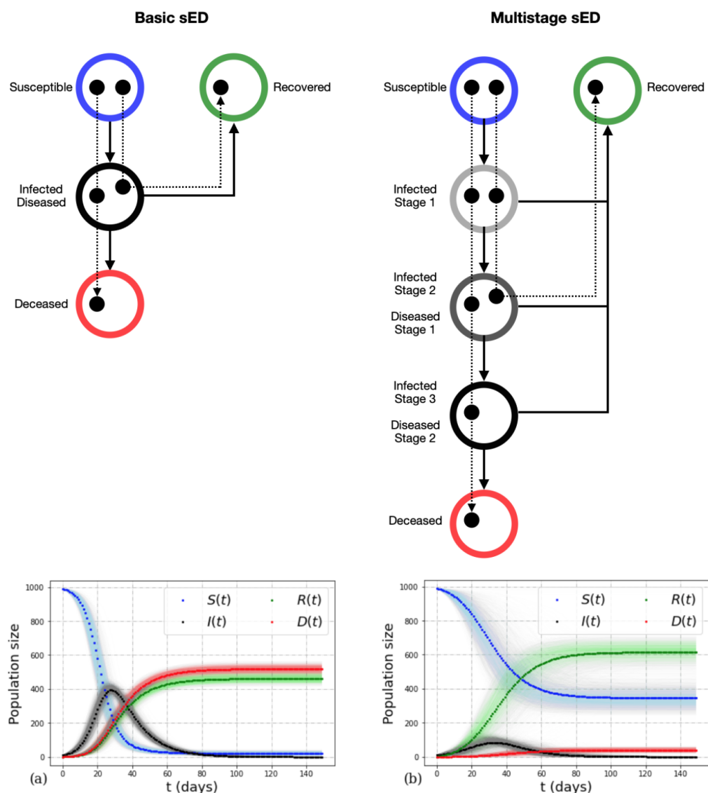
Figure 1: Different dynamical scenarios contemplated by the sED modelling scheme. The light shades represent the confidence intervals generated with 2,000 simulations and the solid dots are taken as the average of those simulations. The two models show different epidemiological dynamics with the same average recovery and death time, but different time courses for infection and disease before recovery or death. See Tables 1 and 2 for further information.
