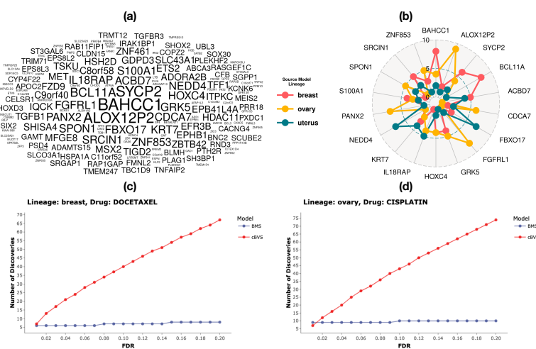
Fig. 3: Drug response model summaries. Panel (a) presents a wordcloud of top genes across all the drug response models (for three lineages and 65 drugs). The sizes of the words are proportional to the total number of times across all models that a gene is selected based on a 10% FDR-controlled threshold. Panel (b) presents a radar chart of the top 18 genes (selected in at least nine out of all the drug response models) according to the three lineages. Panels (c) and (d) present discovery plots across increasing FDR control thresholds for the drug docetaxel in lineage breast and the drug cisplatin in lineage ovary respectively. BMS refers to an uncalibrated Bayesian variable selection model based on the Bayesian model averaging procedure (see Supplementary Notes Section S1.7 ).
