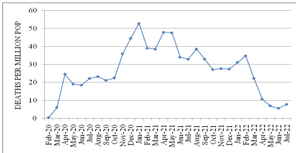
Fig. 2. Time-series of sum monthly deaths cases from Covid-19 per 1 million populations in World from February 2020 to July 2022.
