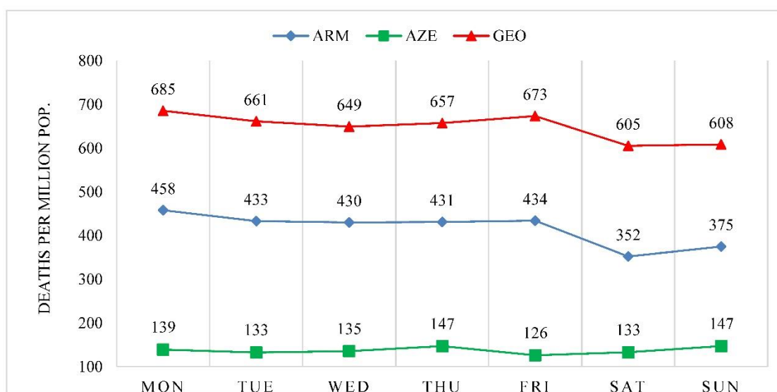
Fig.5. Weekly distribution of sum deaths cases from Covid-19 per 1 million populations in Armenia, Azerbaijan and Georgia from March 2020 to May 2022.
