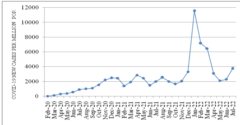
Fig. 1. Time-series of sum monthly Covid-19 new cases per 1 million populations in World from February 2020 to July 2022.
