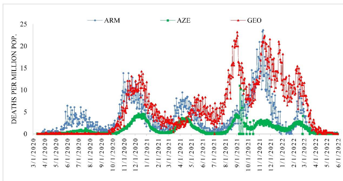
Fig.3. Time-series of daily deaths cases from Covid-19 per 1 million populations in Armenia, Azerbaijan and Georgia from March 12, 2020 to May 31, 2022.
