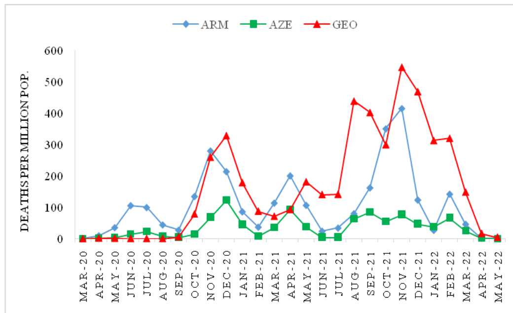
Fig.4. Time-series of sum monthly deaths cases from Covid-19 per 1 million populations in Armenia, Azerbaijan and Georgia from March 2020 to May 2022.
