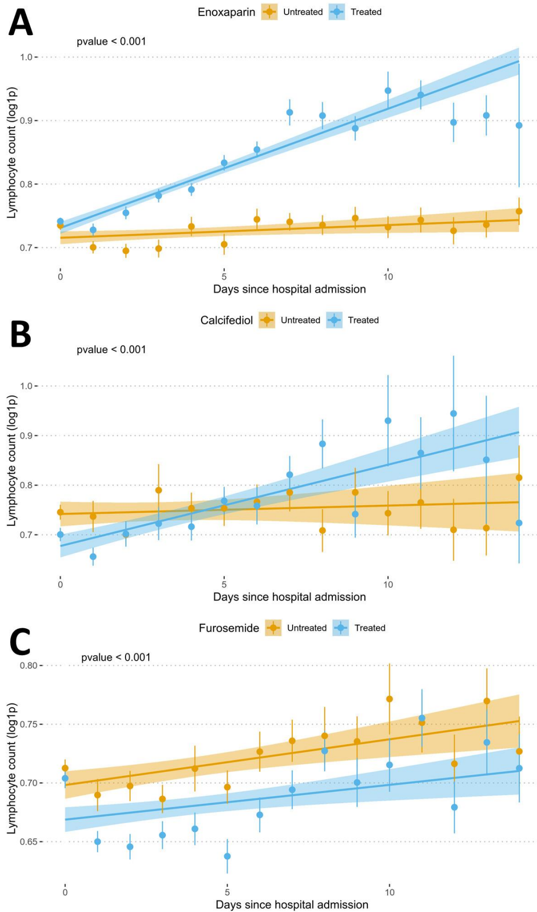
Figure 2. Plots showing the evolution of lymphocyte counts along the time studied (15 days since hospital admission) for A) enoxaparin, B) Calcifediol and C) Furosemide
