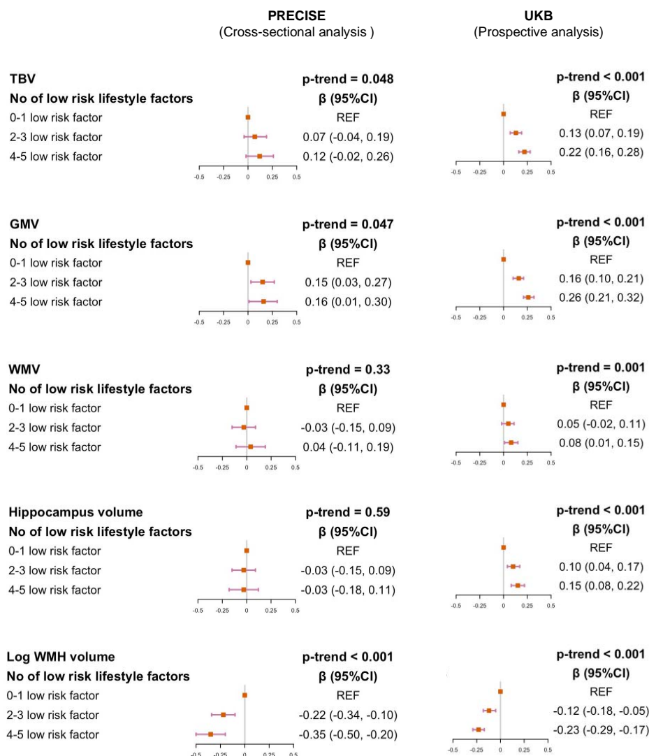
Figure 1 Association between the number of low-risk lifestyle factors and brain MRI markers
