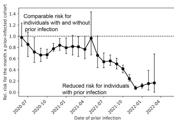
Figure 2: Risk of reinfection over time and relative to the date of prior infection. (a) Relative risk of reinfection during each calendar month, relative to the contemporary rate of first time infections. (b) Relative risk of reinfection during the Omicron era (December 1st, 2021 - May 29, 2022), for individuals with a prior infection during a specific calendar month (x-axis). The dashed horizontal guideline at y=1.0 indicates the expected result when the risk for individuals with a prior infection during the given calendar month (x-axis) is the same as for individuals without prior infection. Error bars indicate 95% confidence intervals.
