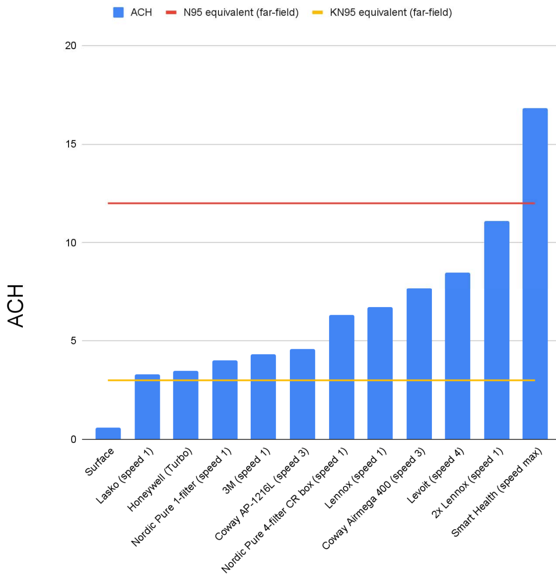
Figure 3: ACH measured for each purifier in single room
