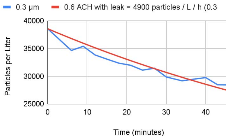
Figure 2: Example of best fit with 7.7 ACH for Coway Airmega 400 in Room
