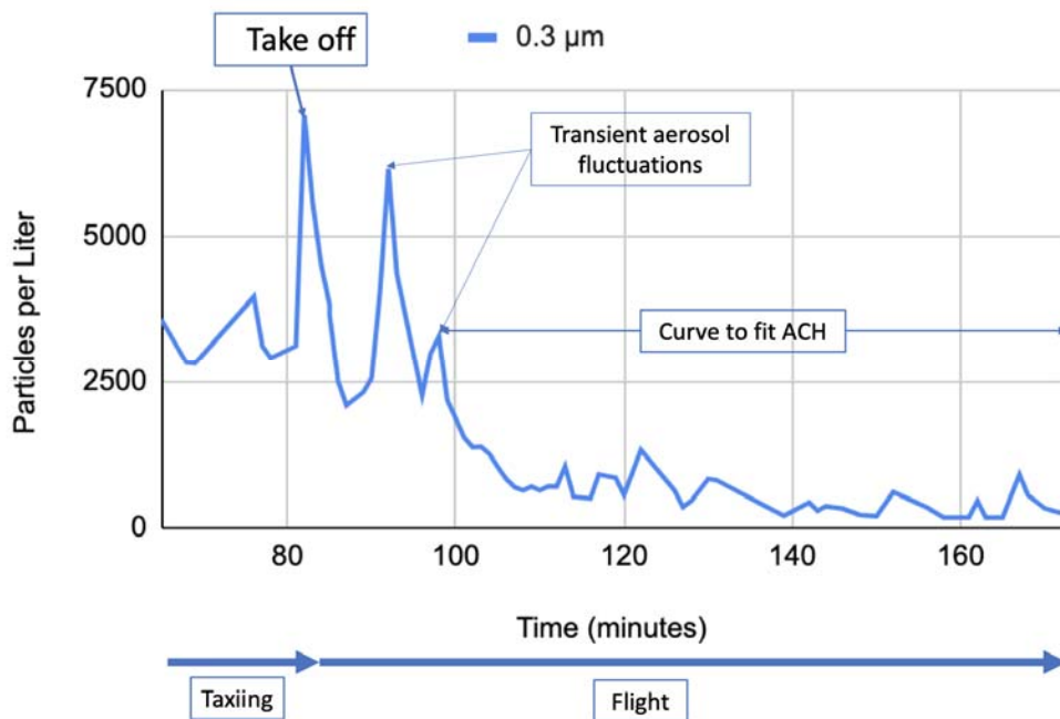
Figure 7: Particle concentration aboard the Airbus A319 during before and after takeoff
