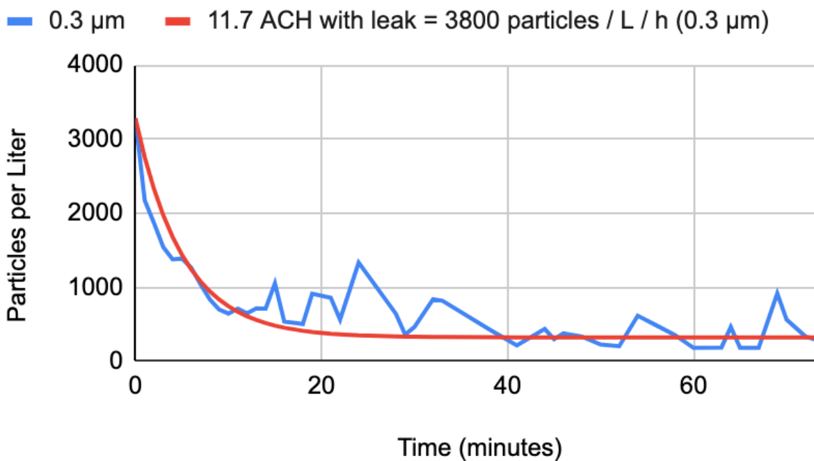
Figure 8: Best fit with 11.7 ACH after takeoff aboard the Airbus A319
