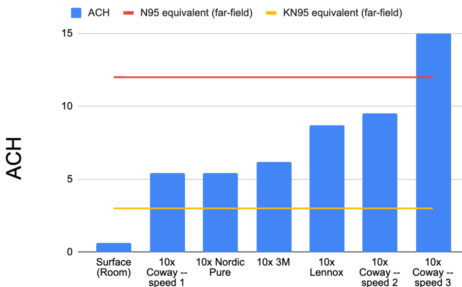
Figure 4: ACH measured for 10 purifiers in whole house
