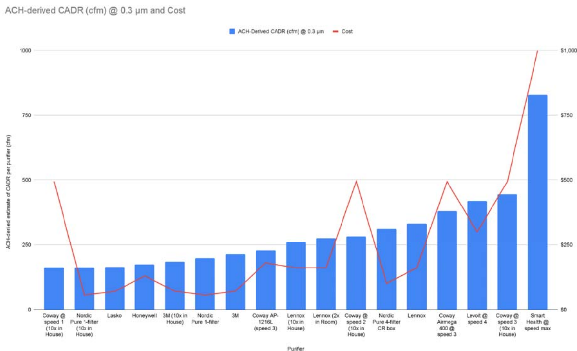
Figure 5: ACH-derived estimate of CADR (cfm) and Cost per purifier
