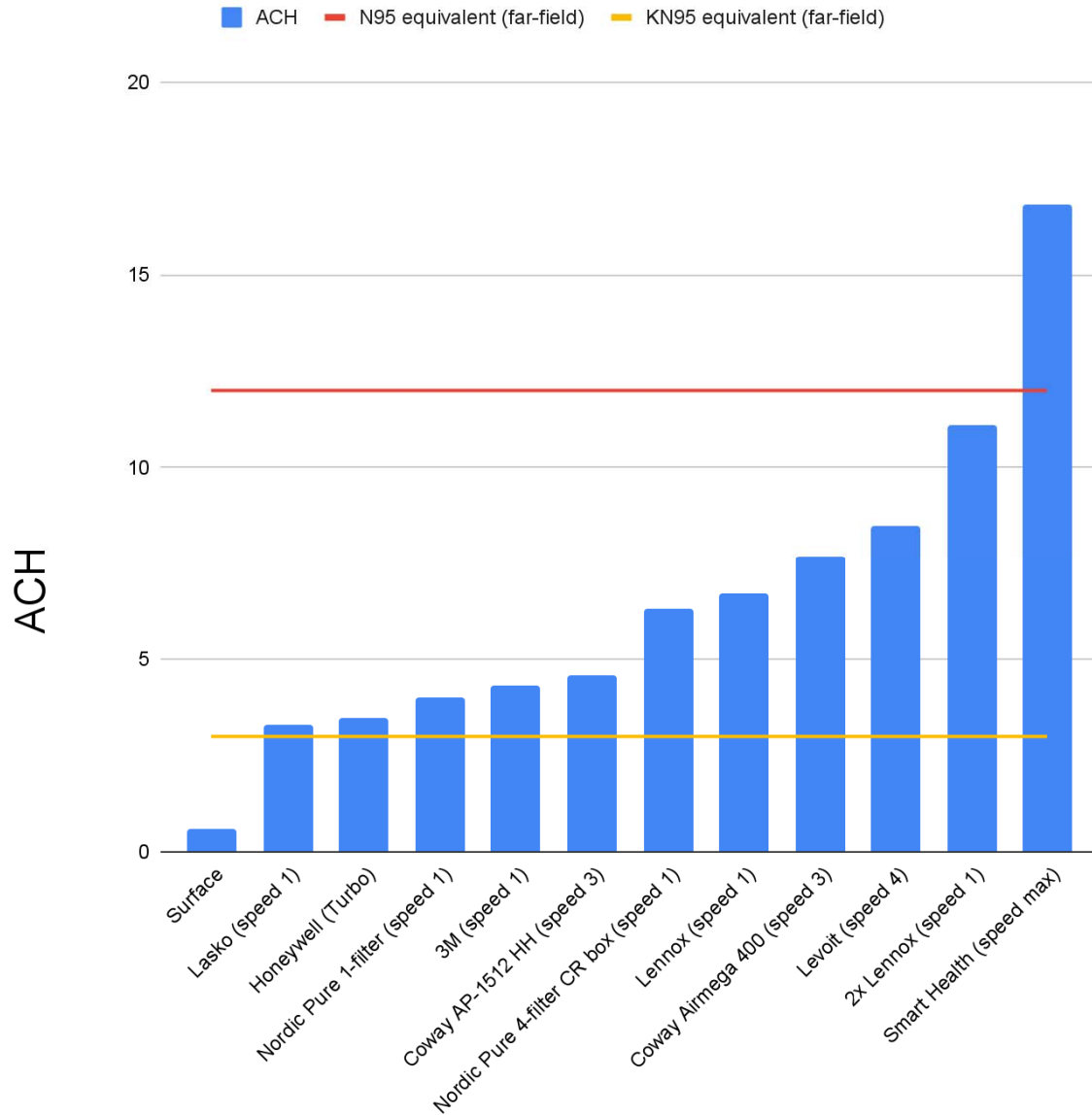
Figure 3: ACH measured for each purifier in single room
