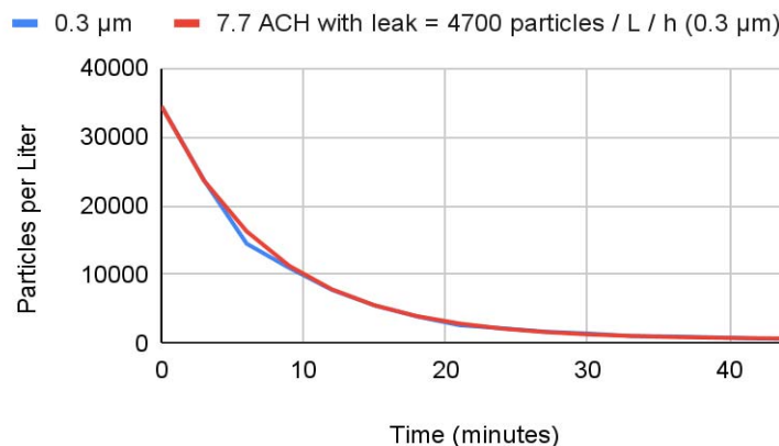
Figure 2: Example of best fit with 7.7 ACH for Coway Airmega 400 in Room
