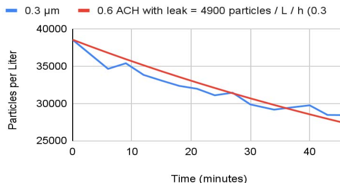
Figure 1: Example of best fit with 0.6 ACH the rate of surface deposition in Room
