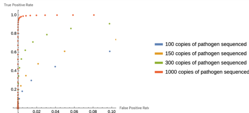
Figure 4: Receiver-operator (ROC) curve for different sequencing depths, 1:30 error rate of sequencing technology and 1:15 ratio of mutated subvariants
