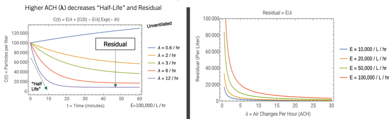
Figure 6: Relationship of Air Changes Per Hour (ACH) to particle concentration
