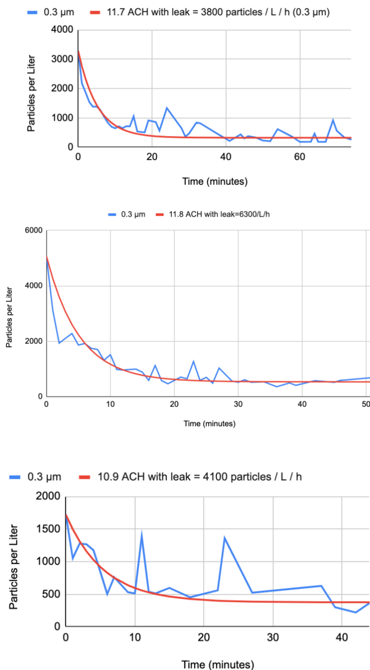
Figure 7: Best fit to estimate ACH after takeoff aboard the Airbus A319, Airbus A321, and Boeing 737-Max8/9
