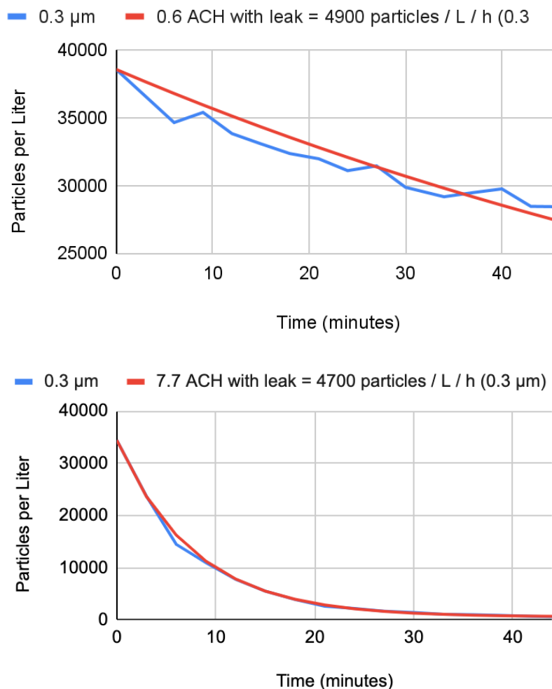
Figure 11: Example of best fit with 0.6 ACH the rate of surface deposition in Room, and best fit with 7.7 ACH for Coway Airmega 400 in Room
