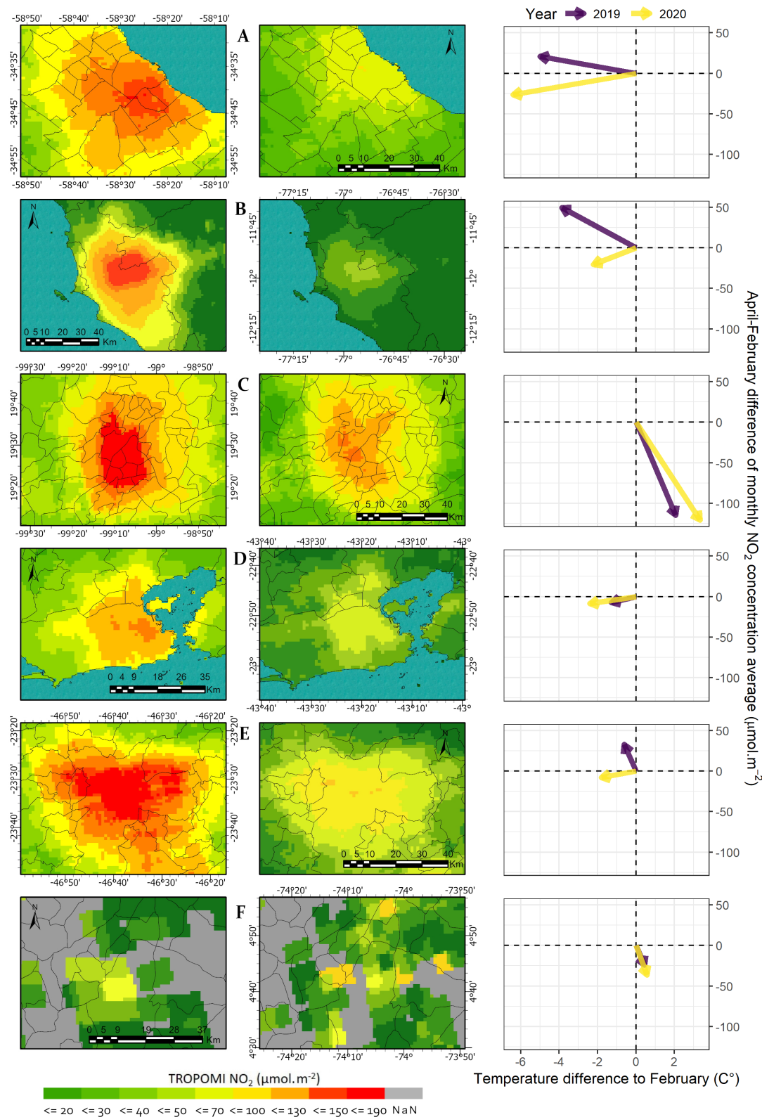
Figure 2: First column: Average tropospheric NO 2 concentration in April 2019. Second column: Average tropospheric NO 2 concentration in April 2020. Third column: 2019 and 2020 April-February differences of tropospheric NO 2 concentration monthly average vs April-February difference of the monthly average temperatures. A) Buenos Aires-Argentina. B) Lima-Perú. C) México DF-México. D) Rio de Janeiro-Brasil. E) São Paulo-Brasil. F) Bogotá-Colombia
