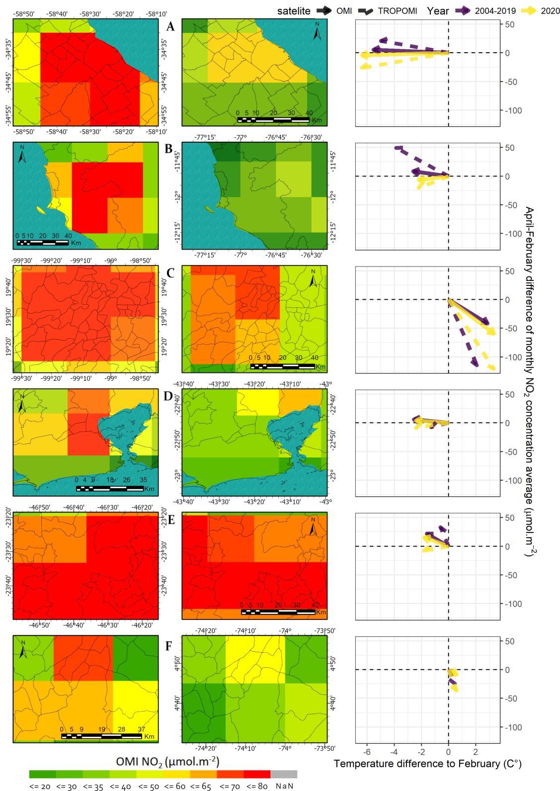
Figure S1: First column: Average OMI's tropospheric NO 2 concentration in April 2019. Second column: Average OMI's tropospheric NO 2 concentration in April 2020. Third column: 2004-2019 average and 2020 April-February differences of tropospheric NO 2 concentration monthly average vs April-February difference of the monthly average temperatures for OMI and TROPOMI's measurements. A) Buenos Aires-Argentina. B) Lima-Perú. C) México DF-México. D) Rio de Janeiro-Brasil. E) São Paulo-Brasil. F) Bogotá-Colombia
