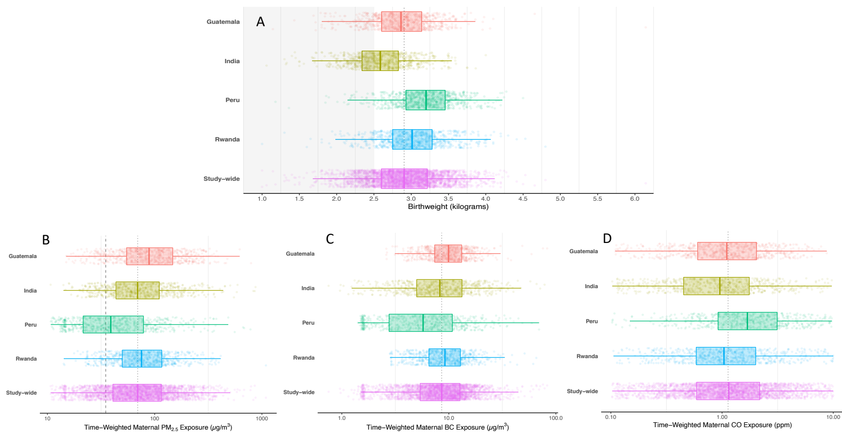
Figure 1. Distribution of (A) birthweight and time-weighted (B) \text{PM}_{2.5} , (C) BC, and (D) CO. Corresponding numeric data are in Supplemental Table 6. Results are presented separately for each study site and in combination for the entire trial. Dots are individual datapoints. X-axes are log transformed. Thick solid lines inside the box are medians. The lower and upper hinges (i.e., the ends of the box) correspond to the 25 th and 75 th percentiles. The whiskers (i.e., the lines beyond the box) extend from the hinge to 1.5 \times \text{IQR} . The panel-wide dotted vertical lines are study-wide medians. In panel (A), the shaded area indicates low birthweight (<math>< 2500\text{ g}</math>). In Panel (B), the dashed line is the WHO Interim Target 1 annual guideline value of 35\ \mu\text{g}/\text{m}^3 .
