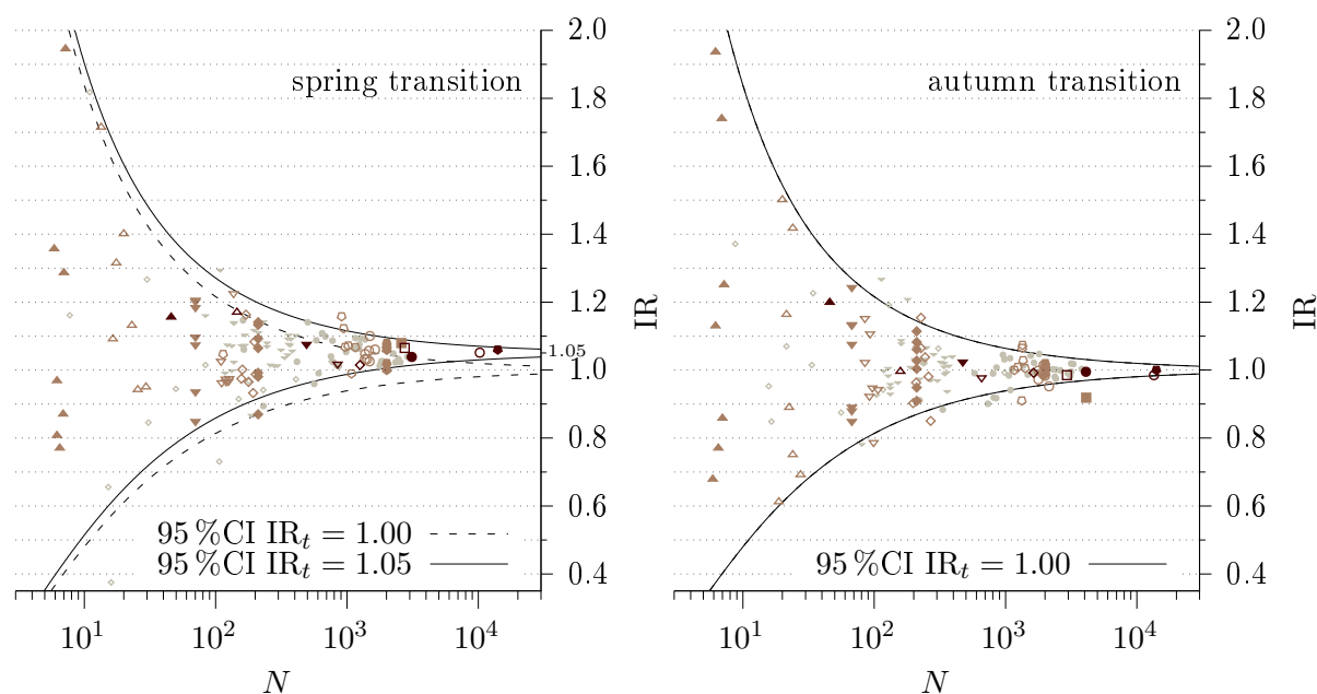
Figure 1 Scatter plot for stratified (lightest ink), day (intermediate ink) and week (darkest ink) IR associated with the spring transition (left panel) and the autumn transition (right panel). The 95 % confidence intervals for selected IR_t are shown. Legend: open circles[2], solid circles[3], open up triangles[4], solid up triangles[5], open down triangles[6], open diamonds[7], solid down triangles[8], solid diamonds[9], open squares[10], solid squares[11], open pentagons[12], solid pentagons[13]. See Table 1 for a breakdown of occurrences inside the 95 % confidence intervals.
