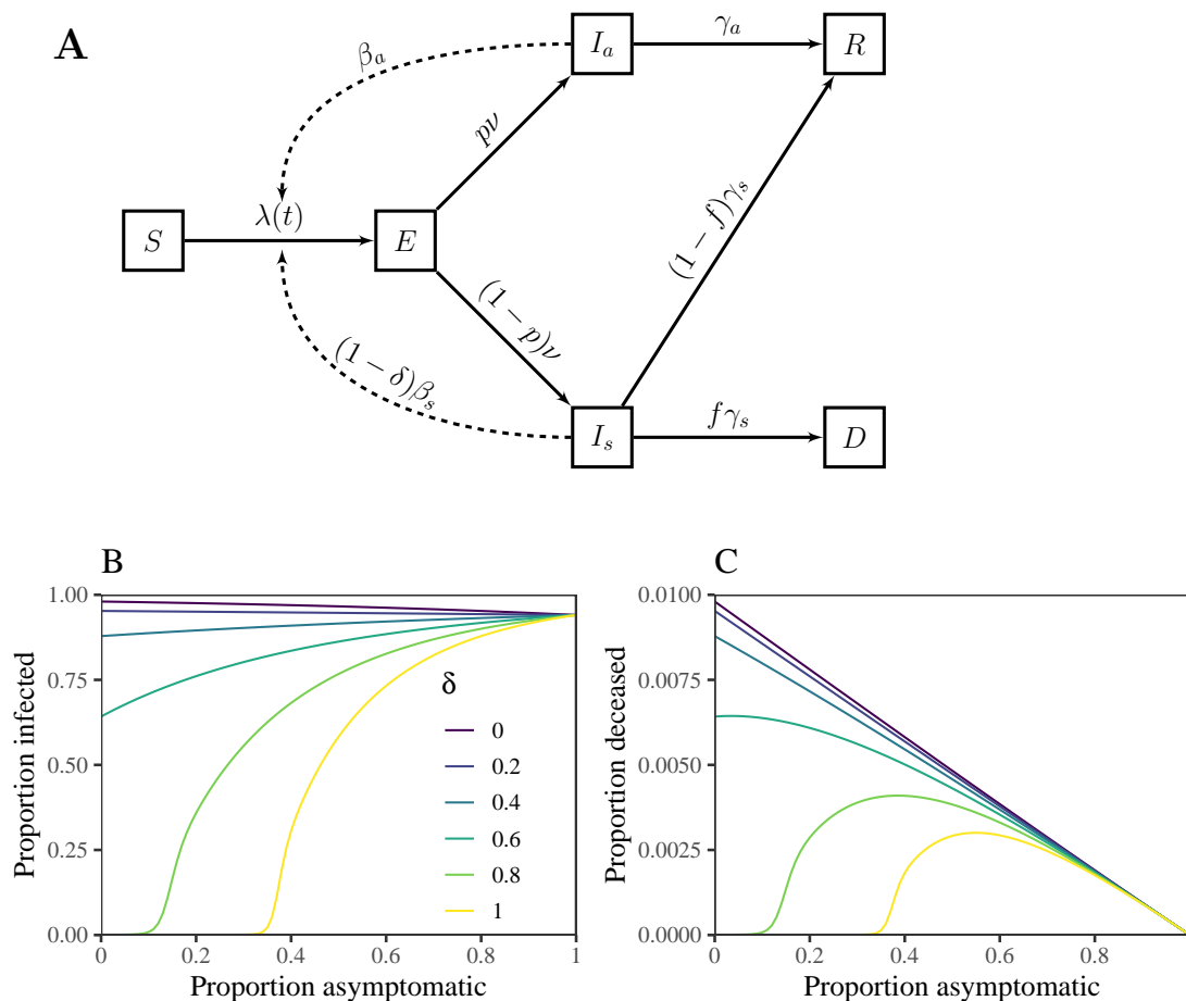
Figure 2: Schematic diagram and simulations of a model with asymptomatic transmission and symptom-responsive transmission reduction. (A) S represents susceptible individuals; E represents exposed individuals; I_a represents asymptomatic individuals; I_s represents symptomatic individuals; R represents recovered individuals; and D represents deceased individuals. See Methods for model details. (B) Total infections as a function of the proportion of asymptomatic infections p across a wide range scenarios for \delta . (C) Total deaths as a function of the proportion of asymptomatic infections p across a wide range scenarios for \delta . We simulate the model for 365 days, assuming \beta_s = 0.8/\text{day} , \beta_a = 0.75\beta_s , \nu = 0.5/\text{day} , \gamma_s = \gamma_a = 0.2/\text{day} , and f = 0.01 , and an initial exposed proportion of 10^{-4} . See Supplementary Text for model details and Supplementary Table S1 for parameter descriptions and values.
