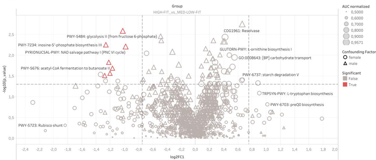
Vulcano plot
