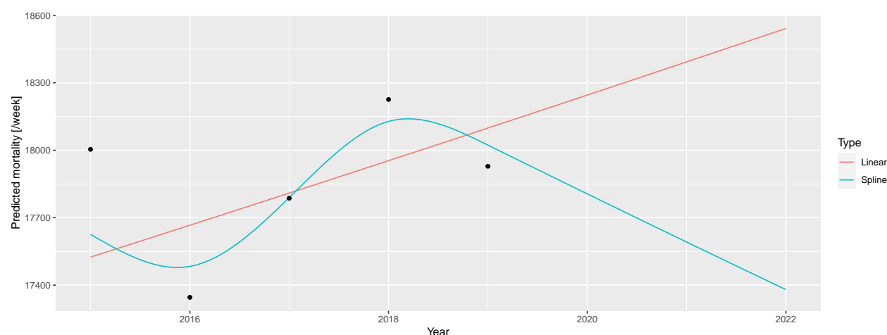
Figure 1: A linear trend and a spline fitted on the 2015–2019 German mortality data and extrapolated to 2020 and 2021.
