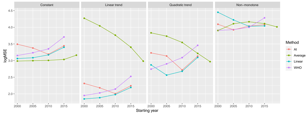
Figure 5: Mean squared errors of the investigated methods by starting year on a logarithmic scale (with k = 3 for the WHO method and \text{tkpy} = 1/7 for the AI approach) for the four defined scenarios.
