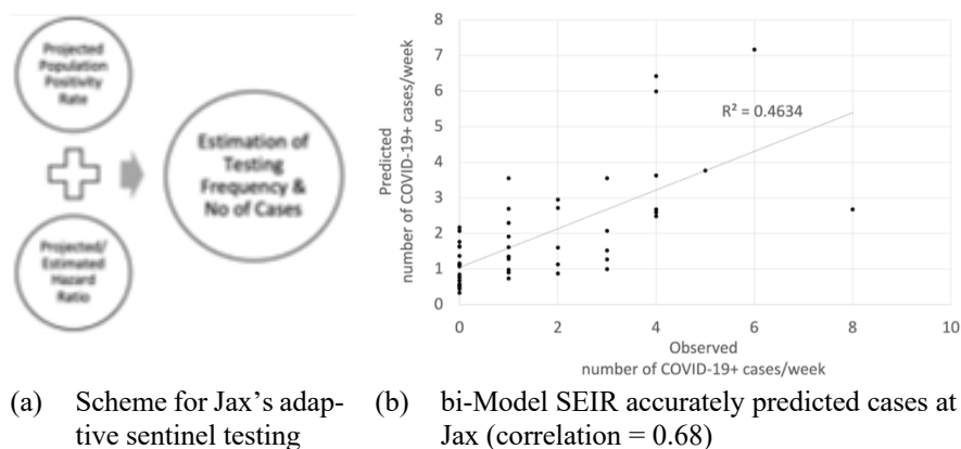
Figure 8: Performance of Bi-Modal SEIR model.
