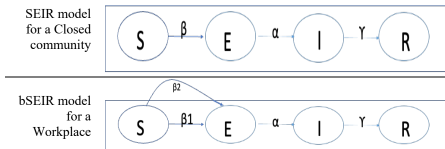
Figure 1: Modeling the pandemic: (top) SEIR model for the closed community, and (bottom) bi-modal SEIR model for the workplace (open system) - \beta_1 and \beta_2 are conversion rates from S to E due to exposure work and at home group respectively.
