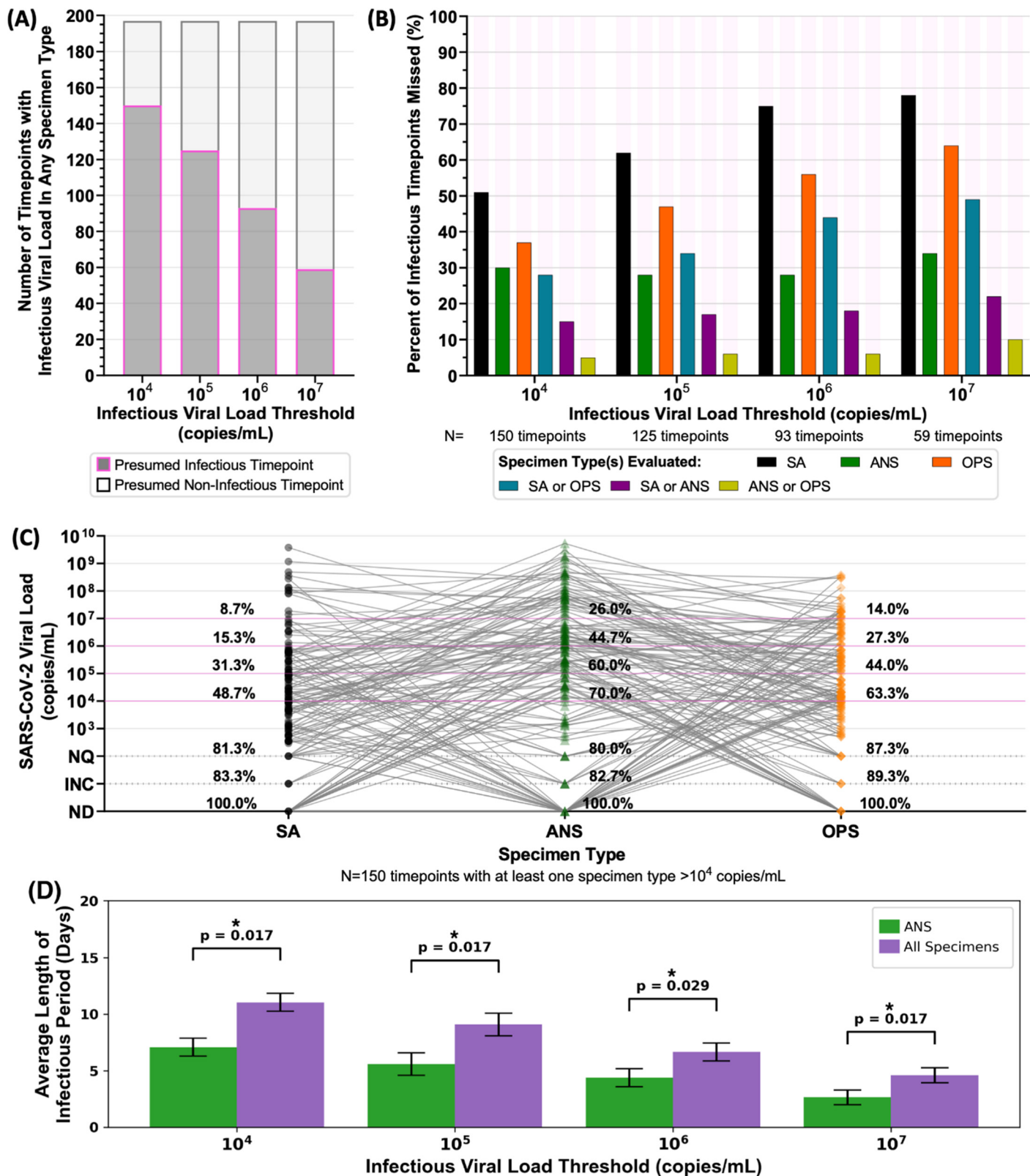
Figure 5. Analyses of Presumed Infectious Viral Loads in Each Specimen Type Using Different Infectious Thresholds. (A) Stacked bar plots of the number of timepoints with at least one specimen type above the indicated infectious viral-load threshold (dark grey with magenta outline), and where all paired specimen types collected at a timepoint had viral loads below the infectious viral-load threshold (light grey with black outline). (B) Each bar represents the proportion of all infectious timepoints (i.e., saliva or nasal swab or throat swab) had a viral load above the infectious viral-load threshold, where the given specimen type or combination of specimen types did not have an infectious viral load. For example, with an infectious viral load threshold of 10^4 copies/mL, 150 timepoints had an infectious viral load in at least one specimen type: in 105 of those 150 timepoints (70%), the ANS specimen had an infectious viral-load. Therefore,
