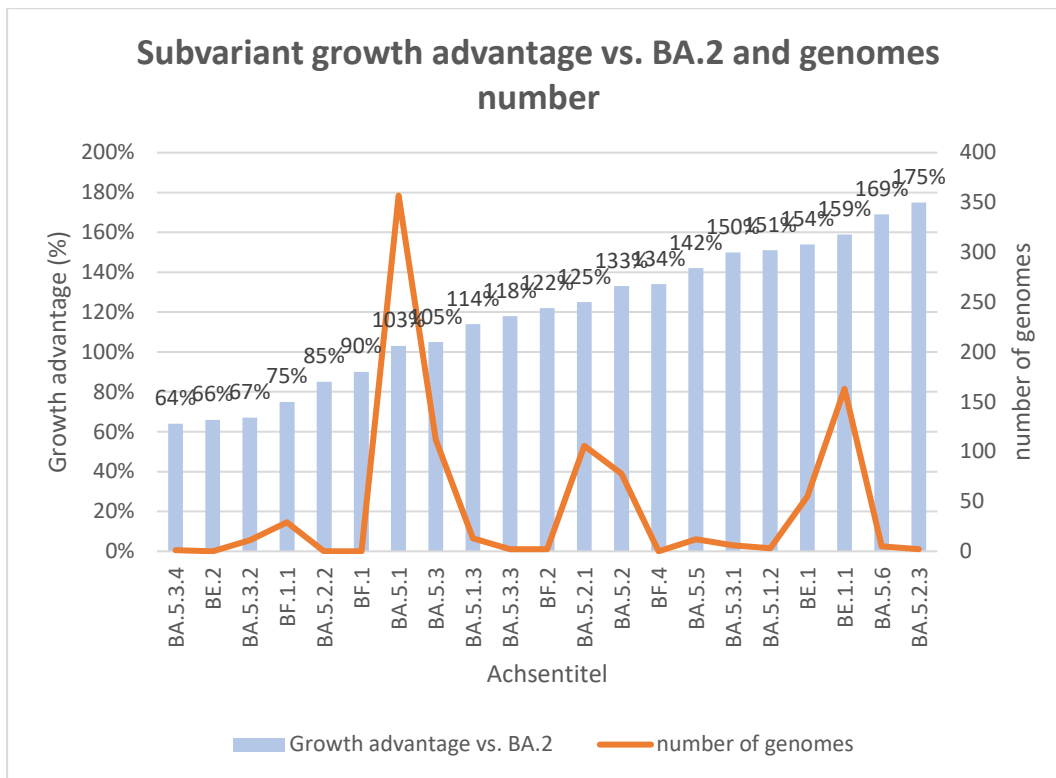
161 Figure 3. Subvariant growth advantage vs. BA.2 and genomes number
