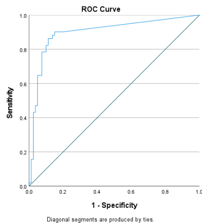
Figure 1a: ROC curve analysis of C. auris real-time PCR assay for patient surveillance samples - Validation samples – AUC 0.89 and optimal cutoff 36.09
