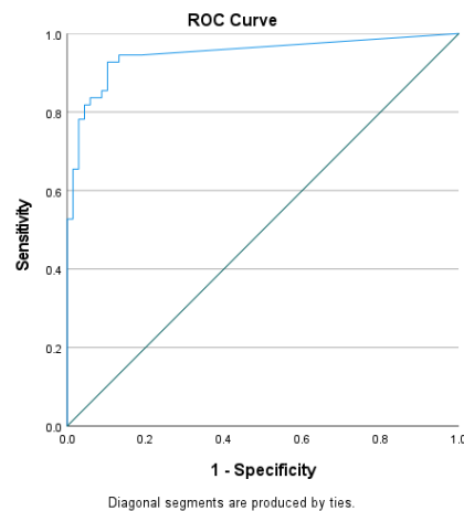
Figure 1b - ROC curve analysis of C. auris real-time PCR assay for patient surveillance samples - Prospective samples – AUC 0.948 and optimal cutoff 36.92
