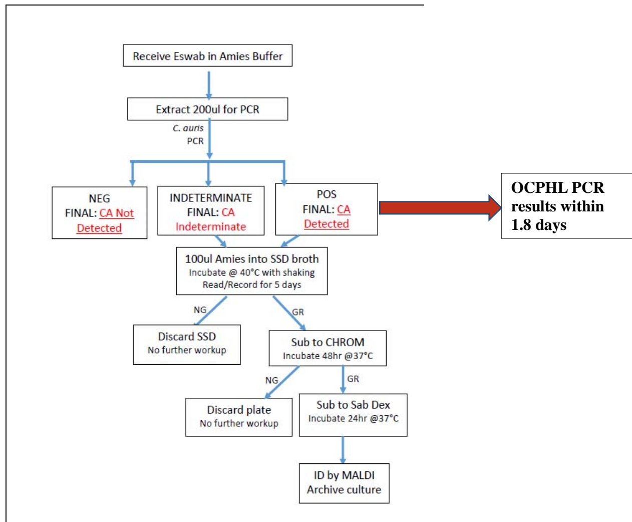
Figure 2: New workflow for C. auris surveillance swabs
