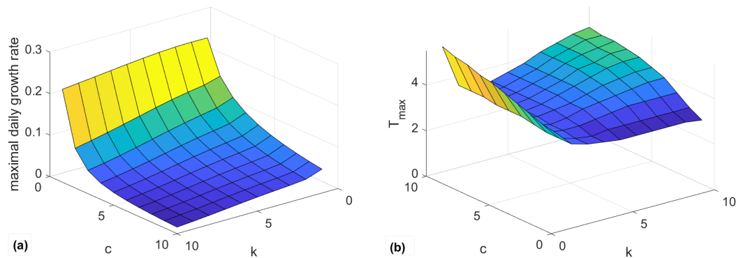
Figure 3. Growth rates and optimal disease durations as a function of c and k . (a) shows the maximal exponential growth rate r of an epidemic pathogen given different values of c and k . We see that growth rates are highest for low c and also decrease slightly with k . (b) shows the optimum disease duration T_{max} . This is equal to the predictions from Eq. (5) for k = 1 and drops as k increases, though for c > 1 there is a minimum value which is reached at k between 1 and 5. \beta is here taken to be 1.
