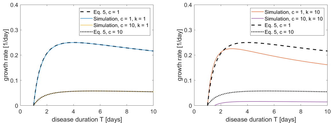
Figure 2. A plot of growth rate as a function of disease duration T as simulated, compared with the growth rate derived in Eq. 5. Here, we set \beta = 1 per day. One observes that the growth rate has a maximum at duration T = \frac{(c+1+2\sqrt{c})c-c^2+3c+2\sqrt{c}}{2c\beta} (equal to 4 for c = 1 and 5.48 for c = 10 ) when using the expression derived theoretically. However, this varies when changing the shape factor k of the probability distribution function of the duration of latent and infectious periods.
