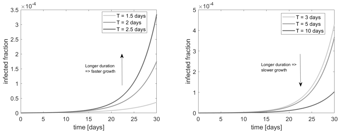
Figure 1. A simple simulation of the initial exponential growth phase of an epidemic given different disease durations T . We see that up to a certain optimum, the disease grows faster for longer durations, but afterwards a longer infectious period leads to slower exponential growth. This illustrates the analytically derived growth rate shown in Fig. 2. Here, \beta = 1 and c = 1 .
