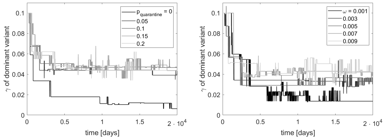
Figure 4. Evolution of variants over time. The figure shows the evolution of the recovery rate \gamma (i.e., the inverse disease duration) of new variants (a) for different quarantine probabilities p , with immunity loss rate set to \omega = 0.01 and (b) for different immunity loss rates \omega with p = 0.1/day . \beta is here set to 0.5 and c = 1 . We see that when people are able to self-quarantine, the variants gradually evolve towards some evolutionarily stable state, whereas this does not appear to be the case if there is no quarantine.
