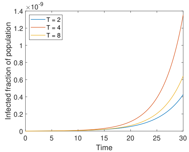
FIG. 1. Direct simulation of the initial growth of an epidemic for different disease durations T . When disease duration is short, the epidemic grows faster as T increases because each infected individual can infect more people. However, for larger values of T , the cost of the longer latent period increases and leads to slower exponential growth. Here, \beta = 1 , k = 1 , and c = \tau/T = 1 , corresponding to assuming equal duration of the E and I states. The initial exposed and infected fractions of the population are E(0) = 10^{-12} and I(0) = 10^{-12} .
