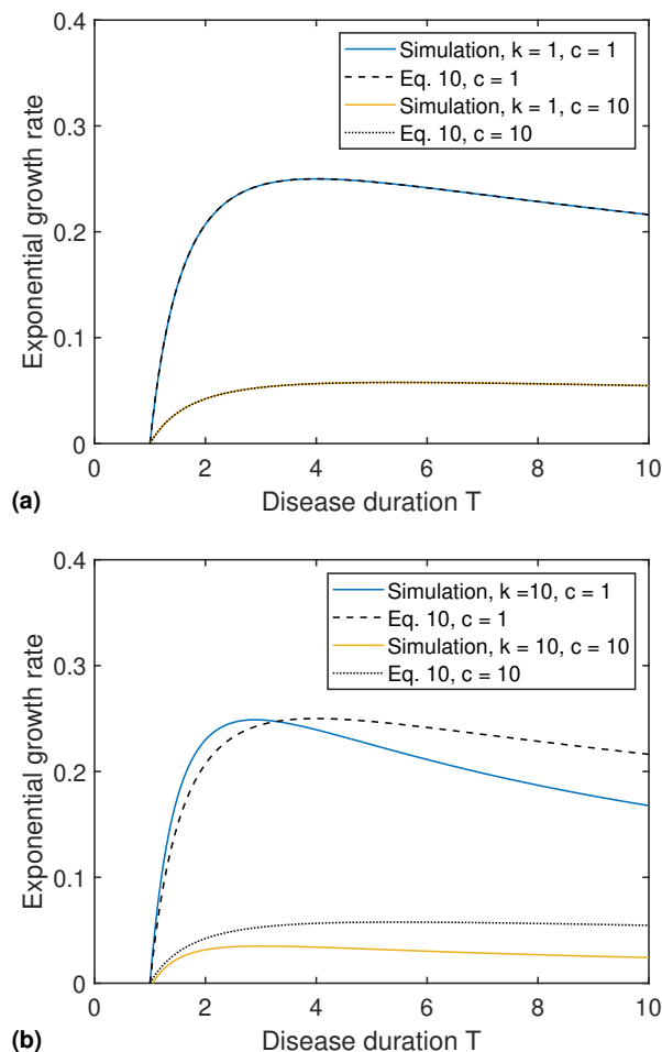
FIG. 2. Growth rate as a function of infectious period duration T as simulated, compared with the growth rate derived in Eq. (10). Here, we set the infection rate \beta = 1/\text{day} . In panel (a) we vary the ratio between exposed and infectious period duration, c . One observes that the growth rate has a maximum at the duration given by Eq. (11) (giving T = 4 for c = 1 and T = 5.48 for c = 10 ). Panel (b) shows the corresponding plot when considering a larger shape factor k for the distribution of the durations of latent and infectious periods.
